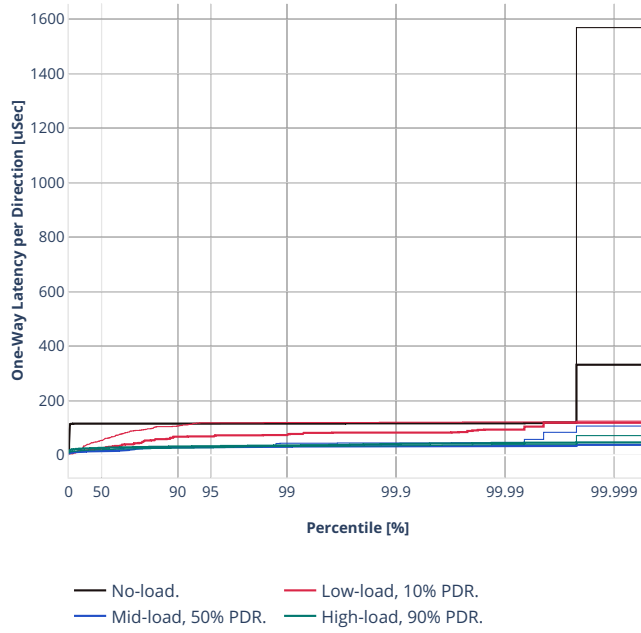
Latency: rdma-eth-l2bdscale10kmaclrn
