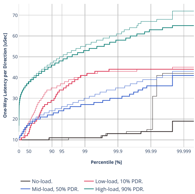
Latency: eth-l2bdscale10kmaclrn
