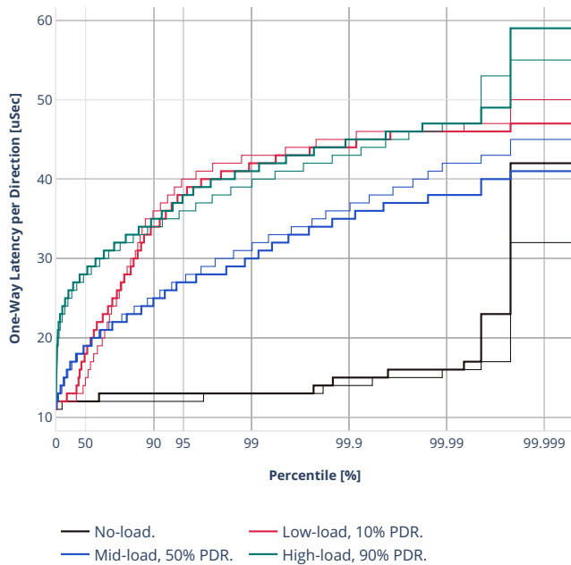
Latency: eth-l2bdscale10kmaclrn
