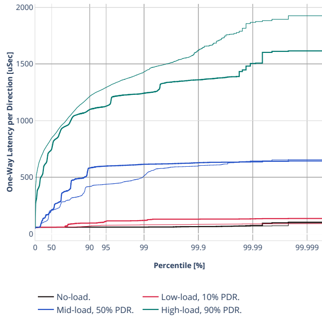
Latency: ethip4ipsec1000tnlhw-ip4base-int-aes128cbc-hmac512sha
