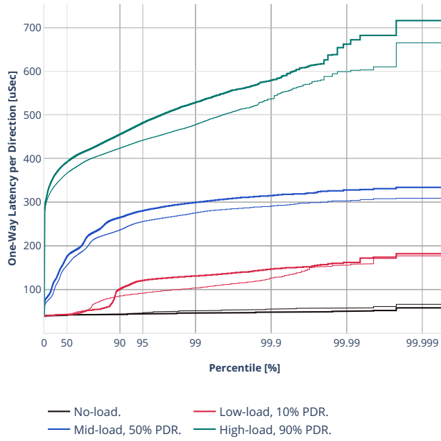
Latency: ethip4-ip4base-eth-2vhostvr1024-1vm-vppip4
