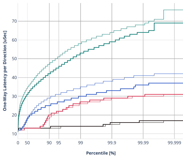
Latency: avf-ethip6-ip6scale2m
