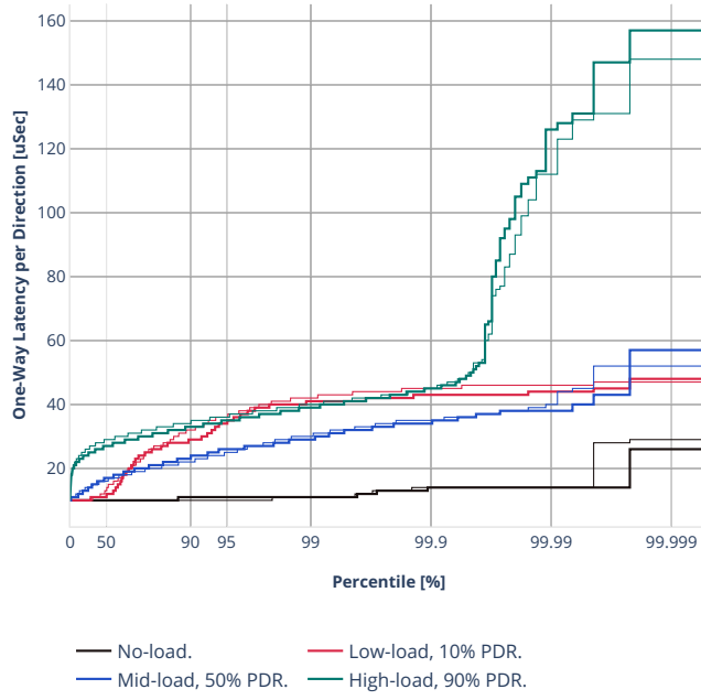
Latency: ethip4-ip4scale200k-rnd
