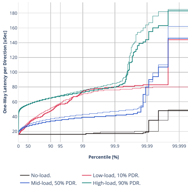
Latency: ethip4-ip4base
