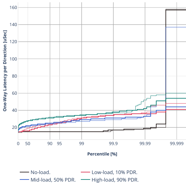
Latency: avf-eth-l2patch
