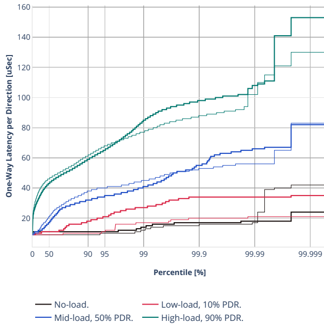
Latency: ethip4udp-ip4base-oacl50sf-10kflows
