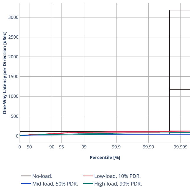
Latency: rdma-eth-l2bdscale1mmaclrn
