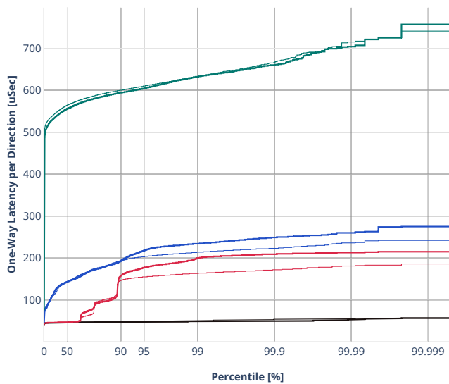
Latency: eth-l2bdbasemaclrn-eth-2memif-1lxc
