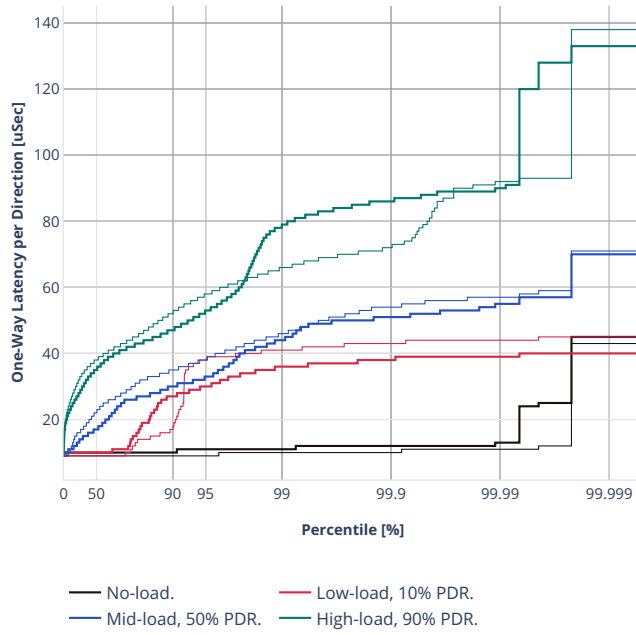
Latency: dot1q-l2bdbasemaclrn
