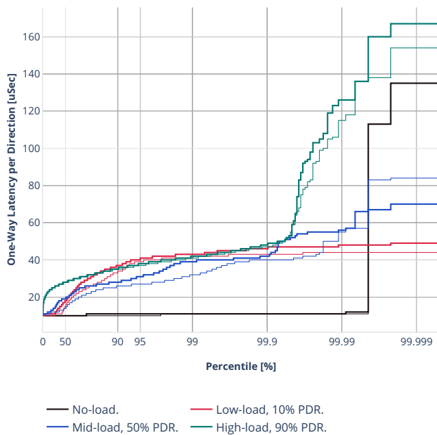
Latency: ethip4-ip4scale2m-rnd
