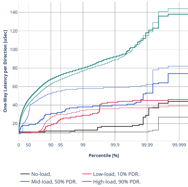
Latency: eth-l2bdbasemaclrn-oac150sl-10kflows
