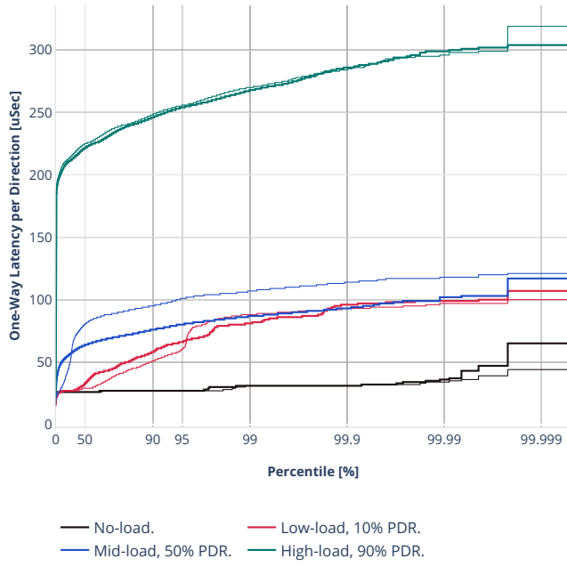
Latency: ethip6srhip6-ip6base-srv6proxy-masq
