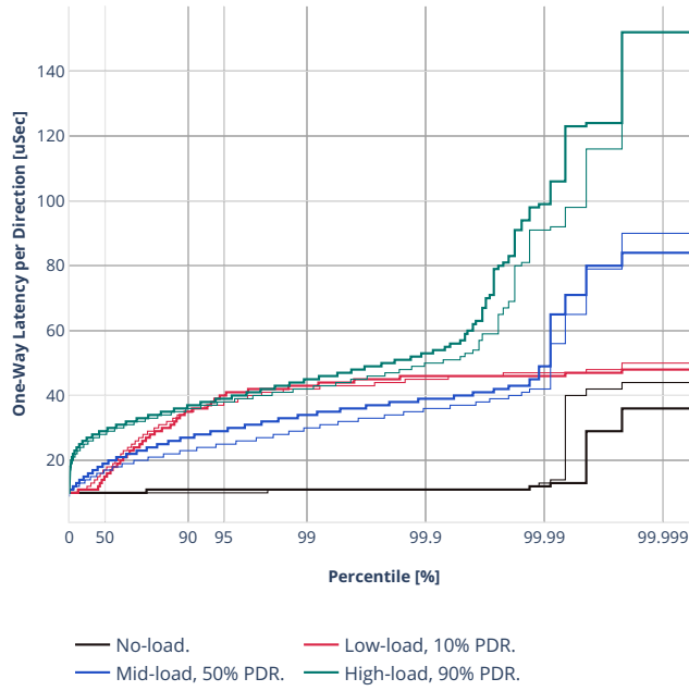
Latency: ethip4-ip4scale2m
