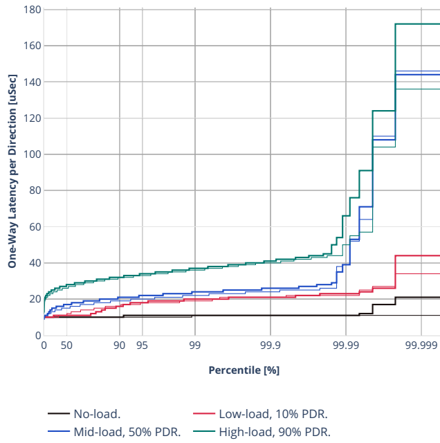
Latency: avf-ethip4-ip4base
