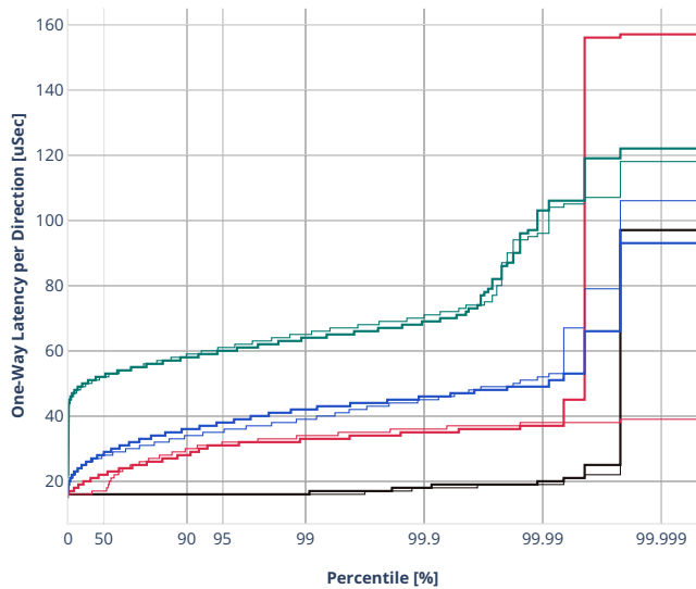
Latency: avf-ethip4-ip4base
