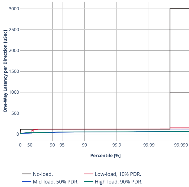
Latency: rdma-ethip4udp-nat44det-h1-p1-s1
