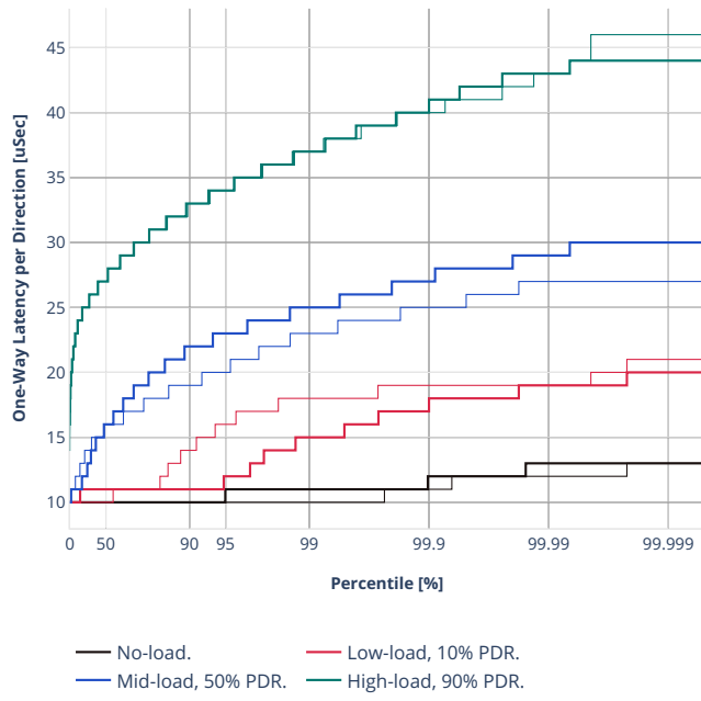
Latency: avf-ethip4-ip4base
