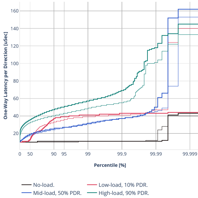
Latency: eth-l2bdscale1mmaclrn
