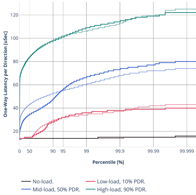
Latency: avf-eth-l2bdbasemaclrn-eth-2memif-1dcr
