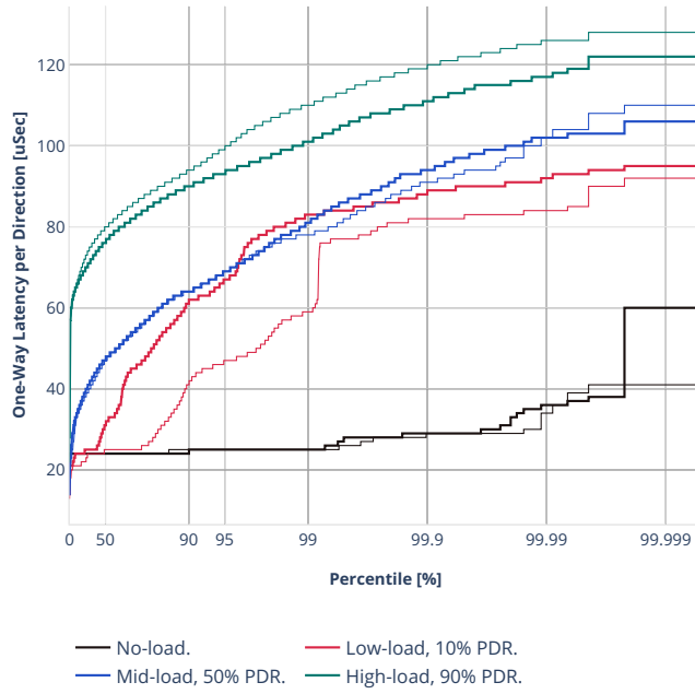
Latency: ethip6srhip6-ip6base-srv6enc2sids
