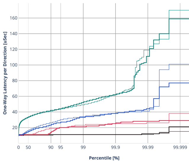
Latency: avf-ethip6-ip6scale2m-rnd
