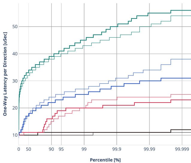
Latency: avf-eth-l2bdscale100kmac1rn
