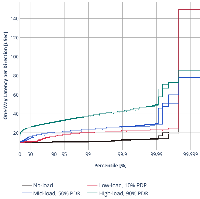
Latency: avf-ethip4-ip4scale200k
