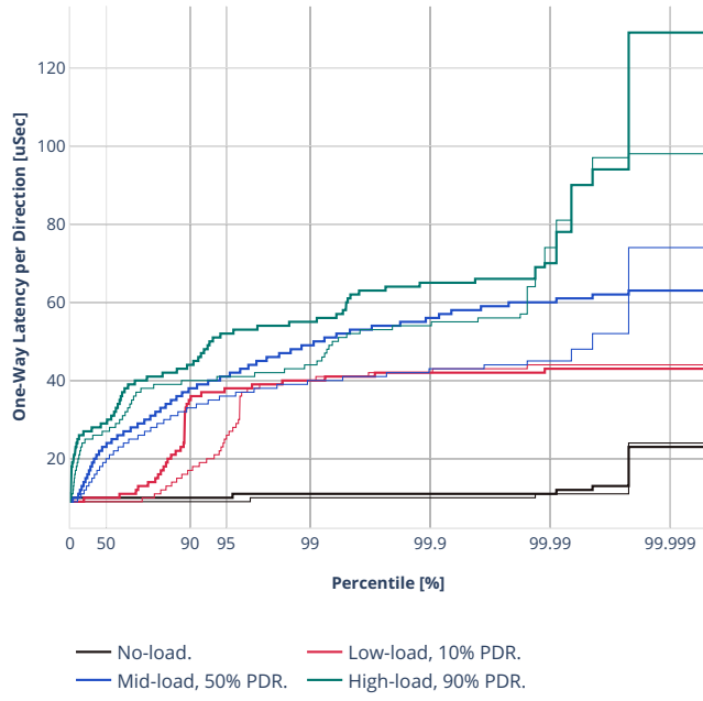
Latency: ethip6-ip6base
