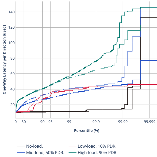
Latency: ethip6-ip6scale2m
