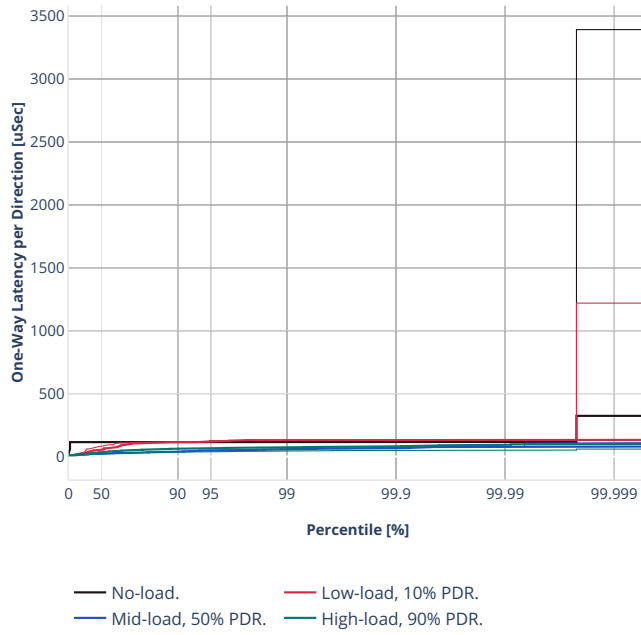
Latency: rdma-ethip4udp-nat44det-h1024-p63-s64512
