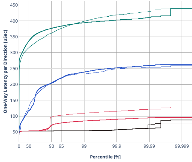
Latency: ethip4ipsec1000tnlhw-ip4base-int-aes256gcm
