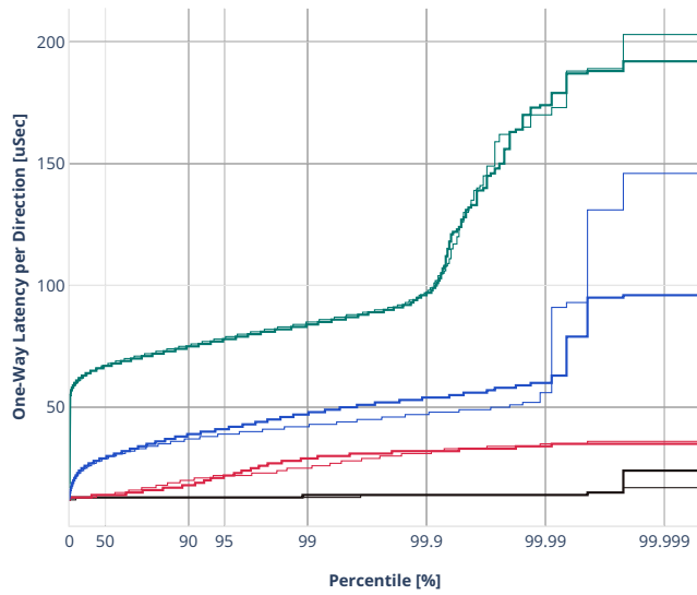
Latency: avf-eth-l2xcbase-eth-2memif-1dcr
