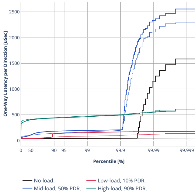
Latency: ethip6srhip6-ip6base-srv6proxy-masq
