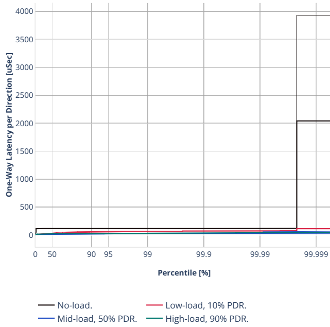
Latency: rdma-ethip4-ip4scale200k
