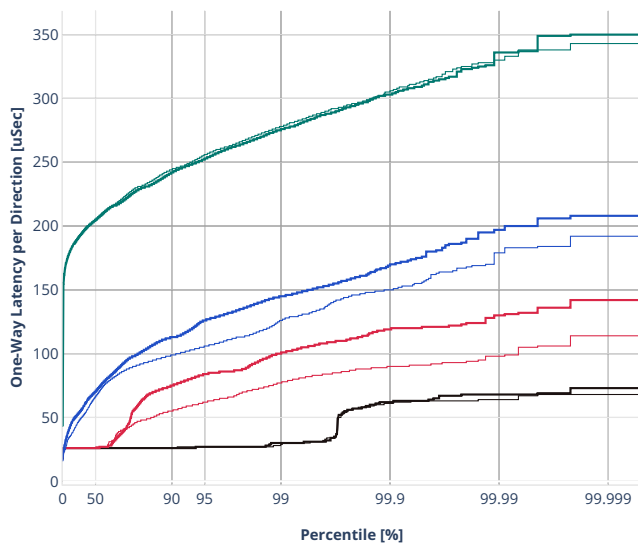
Latency: eth-l2xcbase-eth-2vhostvr1024-1vm
