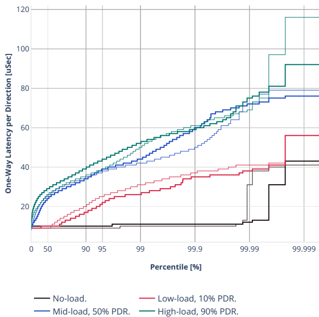
Latency: ethip4-ip4base
