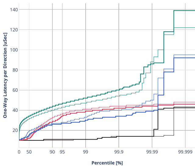
Latency: eth-l2bdscale100kmacirn
