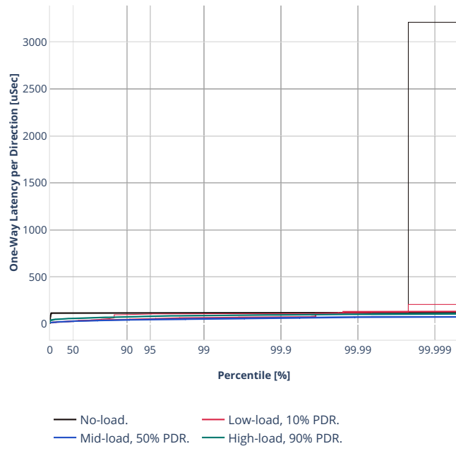
Latency: rdma-ethip4-ip4base-eth-2memif-1dcr
