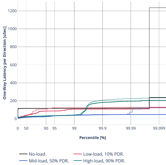
Latency: rdma-ethip6-ip6scale200k-rnd
