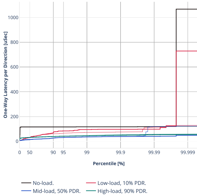
Latency: rdma-dot1q-l2bdbasemacrln
