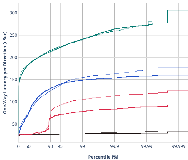
Latency: ethip6srhip6-ip6base-srv6enc2sids
