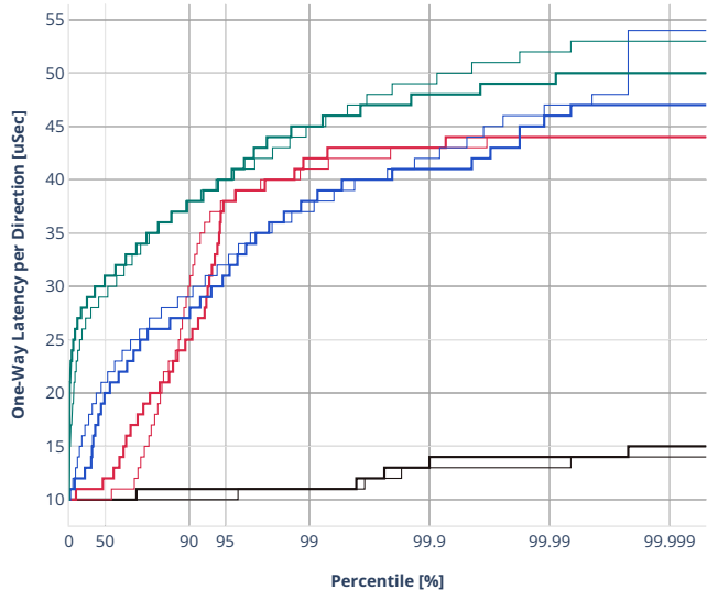
Latency: ethip6-ip6scale20k
