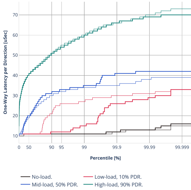
Latency: avf-ethip4udp-ip4base-oac150sl-10kflows
