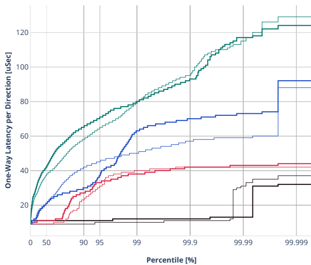
Latency: ethip4udp-ip4base-oacl50sl-10kflows
