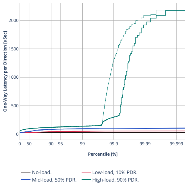
Latency: eth-l2bdbasemaclrn-iac150sl-10kflows
