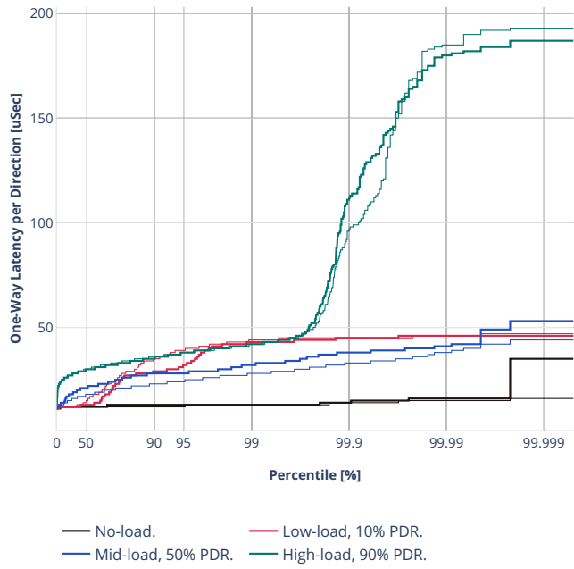
Latency: ethip4-ip4scale2m
