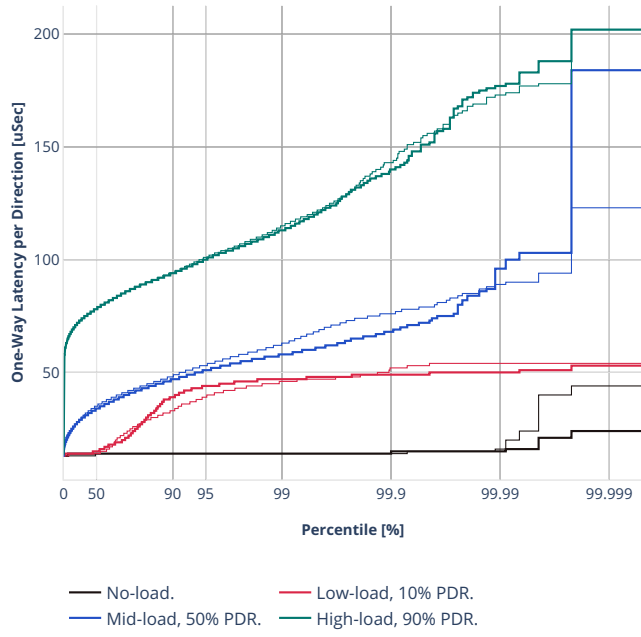
Latency: eth-l2bdbasemaclrn-eth-2memif-1dcr
