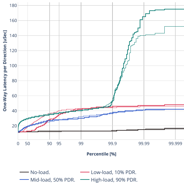
Latency: ethip4-ip4scale200k
