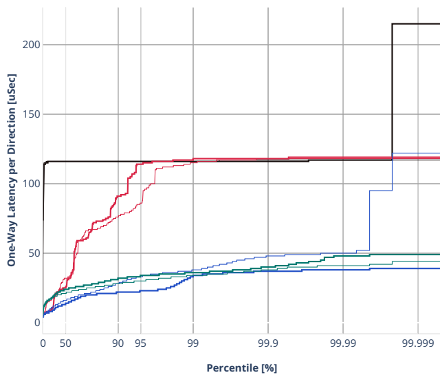
Latency: rdma-ethip4-ip4scale2m-rnd
