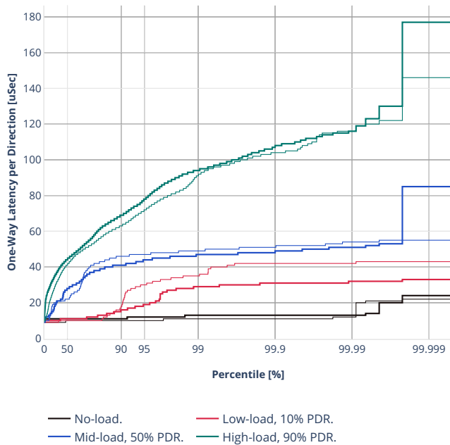
Latency: eth-l2bdbasemaclrn-macip-iac150sl-10kflows
