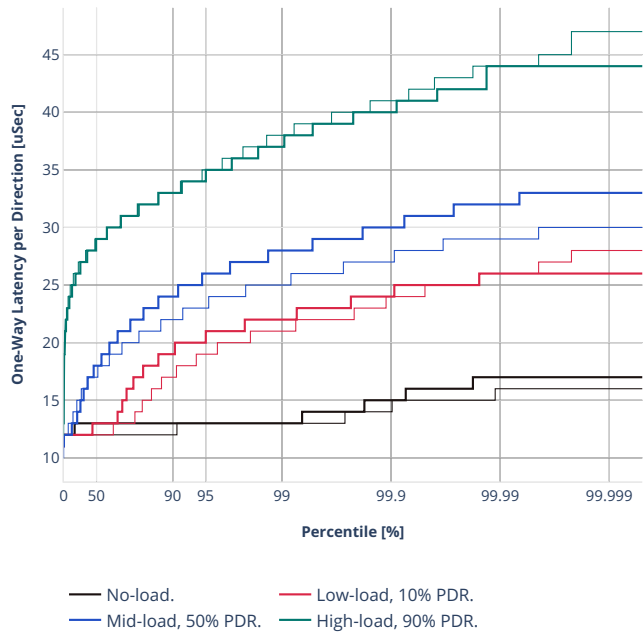
Latency: avf-eth-l2bdscale10kmaclrn
