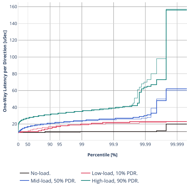
Latency: avf-eth-l2bdbasemaclrn
