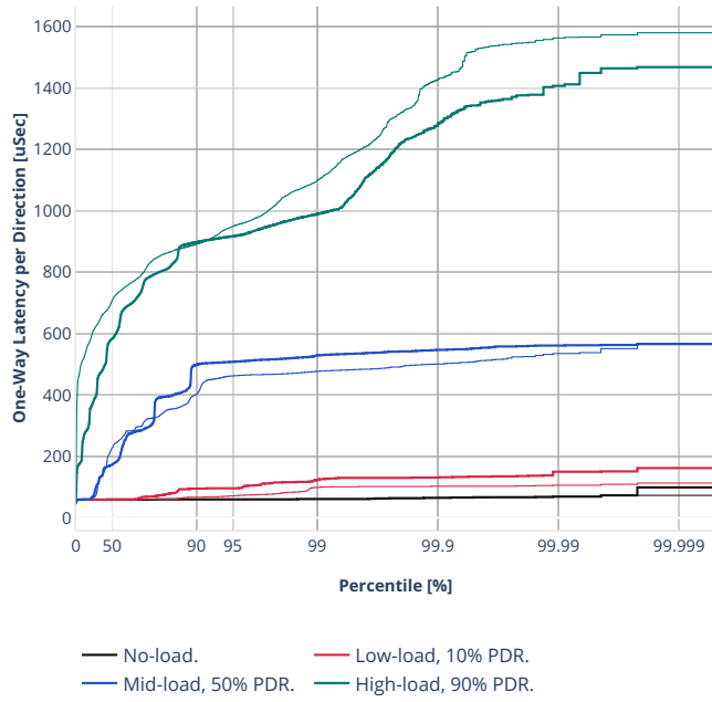
Latency: ethip4ipsec1000tnlsw-ip4base-int-aes128cbc-hmac512sha
