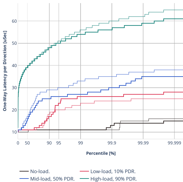
Latency: avf-ethip4udp-ip4base-oac150sf-10kflows
