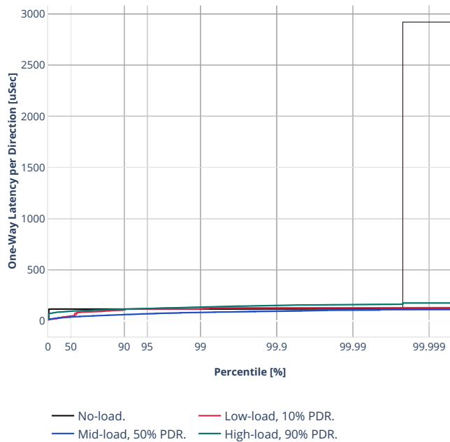
Latency: rdma-eth-l2bdbasemaclrn-eth-2vhostvr1024-1vm
