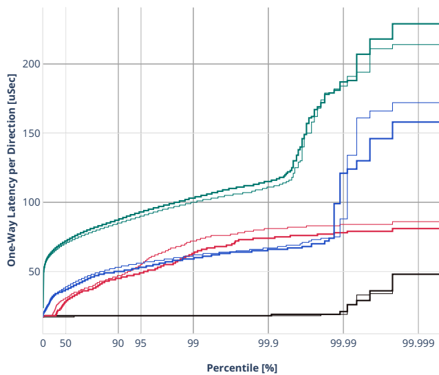
Latency: ethip4vxlan-l2bdbasemaclrn
