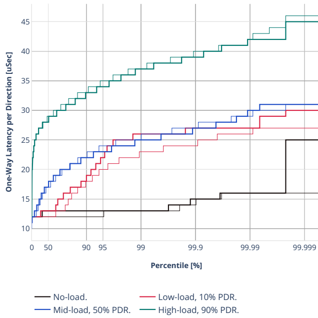
Latency: avf-ethip4-ip4base
