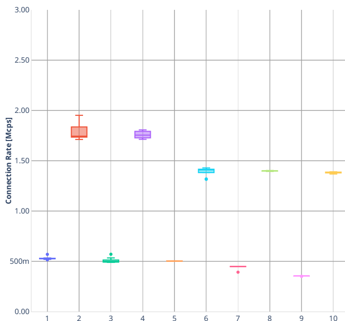
CPS: 2n-clx-xxv710-64b-2t1c-nat44ed-ip4routing-tcp-stf-cps-avf
