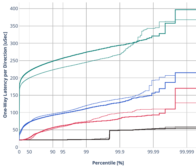
Latency: ethip4-ip4base-eth-2vhostvr1024-1vm
