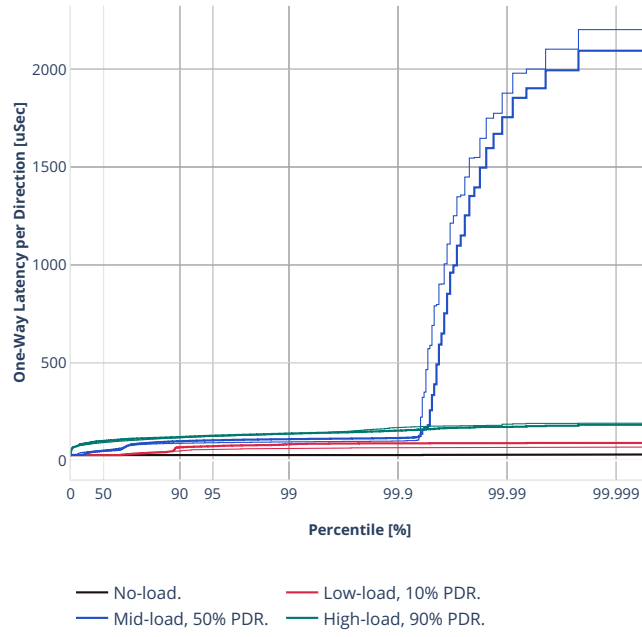
Latency: eth-l2bdbasemaclrn-oac150sf-10kflows
