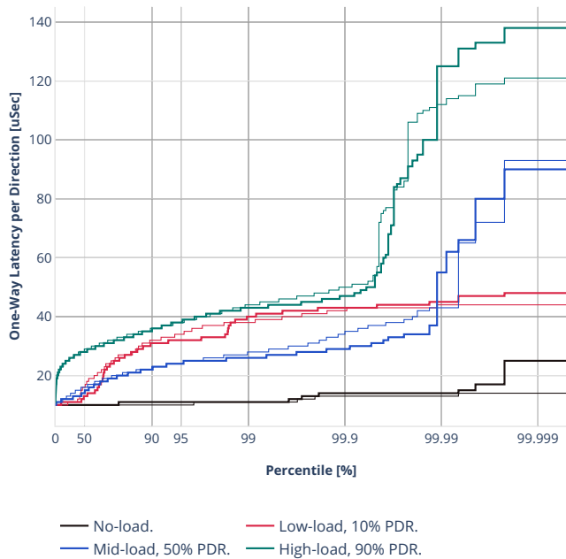
Latency: ethip6-ip6scale20k
