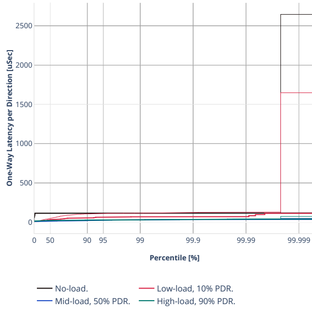
Latency: rdma-eth-l2bdbasemaclrn
