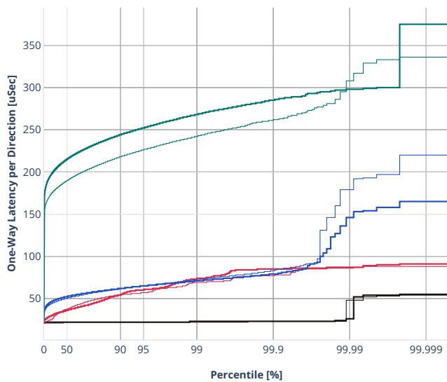
Latency: eth-l2xcbase-eth-2memif-1lxc
