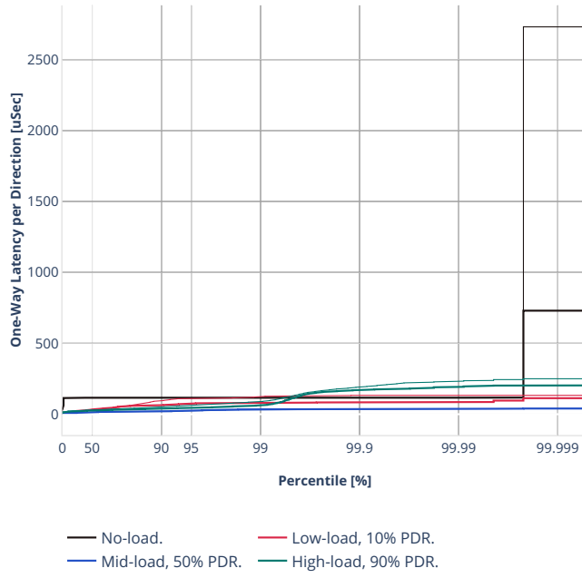
Latency: rdma-ethip6-ip6scale200k
