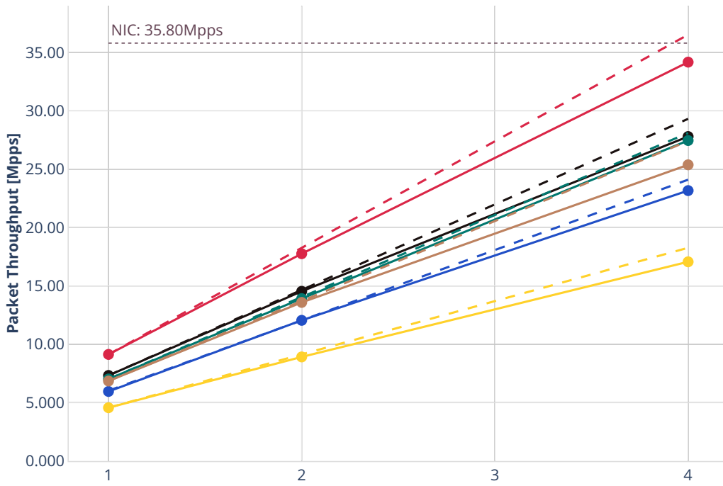
- - Perfect — Measured ··· Limit ● avf-dot1q-l2xcbase-eth-2vhostvr1024-1vm-vppl2xc ● avf-eth-l2xcbase-eth-2vhostvr1024-1vm-vppl2xc ● avf-dot1q-l2bdbasemaclrn-eth-2vhostvr1024-1vm-vppl2xc ● avf-eth-l2bdbasemaclrn-eth-2vhostvr1024-1vm-vppl2xc ● avf-ethip4-ip4base-eth-2vhostvr1024-1vm-vppip4 ● avf-ethip4vxlan-l2bdbasemaclrn-eth-2vhostvr1024-1vm-vppl2xc
