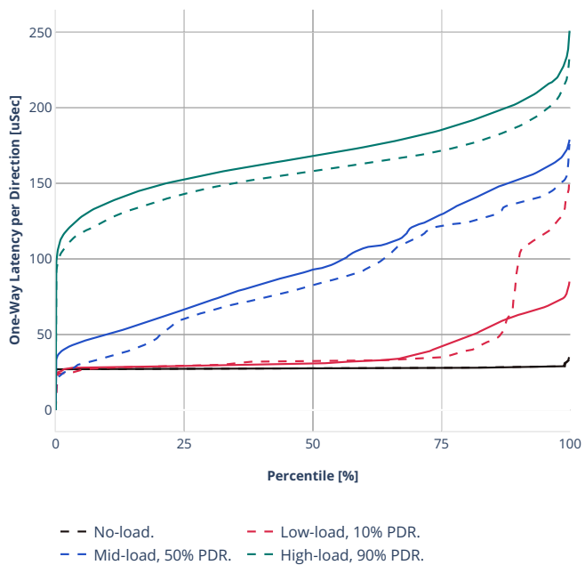
Latency: ethip4-ip4base-eth-2vhostvr1024-1vm-vppip4
