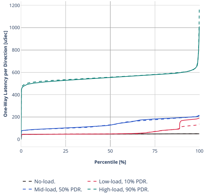
Latency: eth-l2bdbasemaclrn-eth-2memif-1lxc
