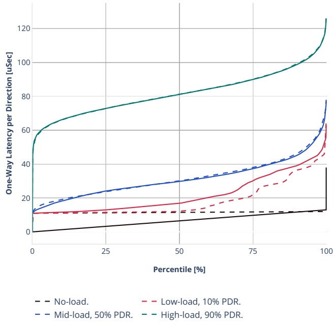
Latency: eth-l2xcbase-eth-2vhostvr1024-1vm
