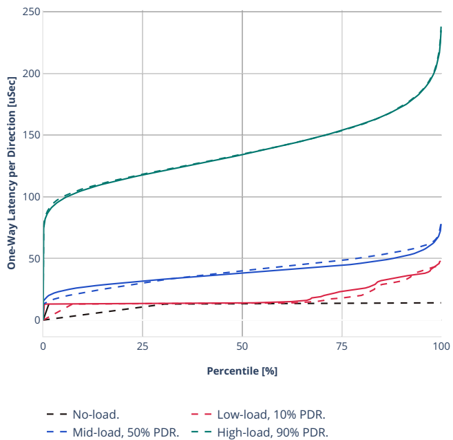
Latency: ethip4-ip4base-eth-2memif-1 dcr
