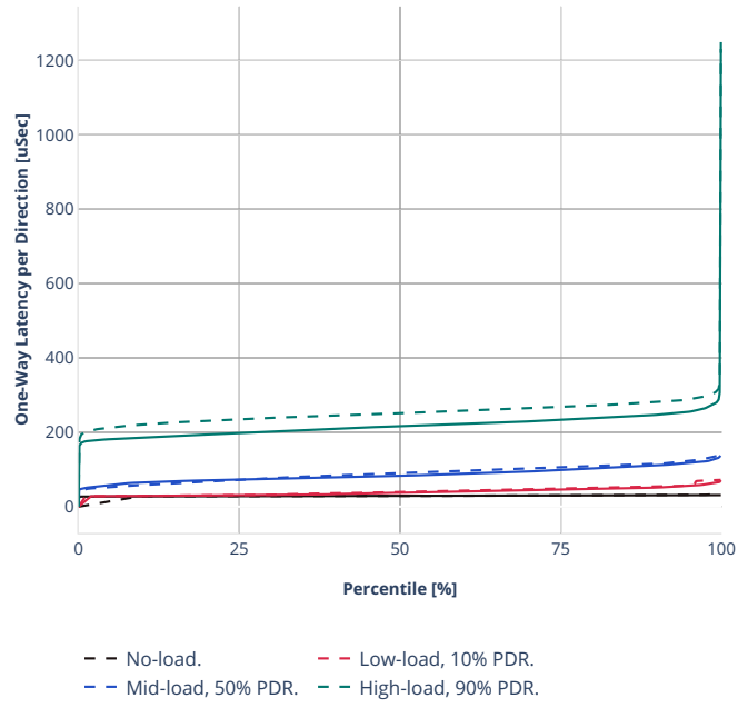
Latency: ethip4vxlan-l2bdbasemaclrn
