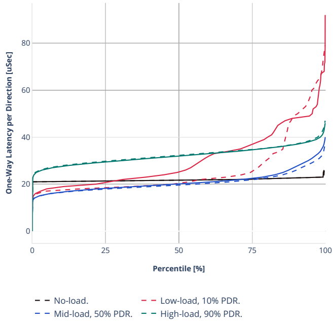
Latency: eth-l2patch
