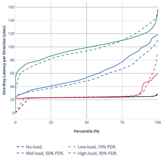
Latency: ethip4udp-ip4base-oac150sl-10kflows
