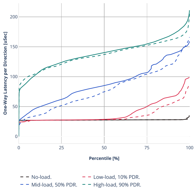
Latency: eth-l2bdbasemaclrn-eth-2vhostvr1024-1vm-vpp12xc
