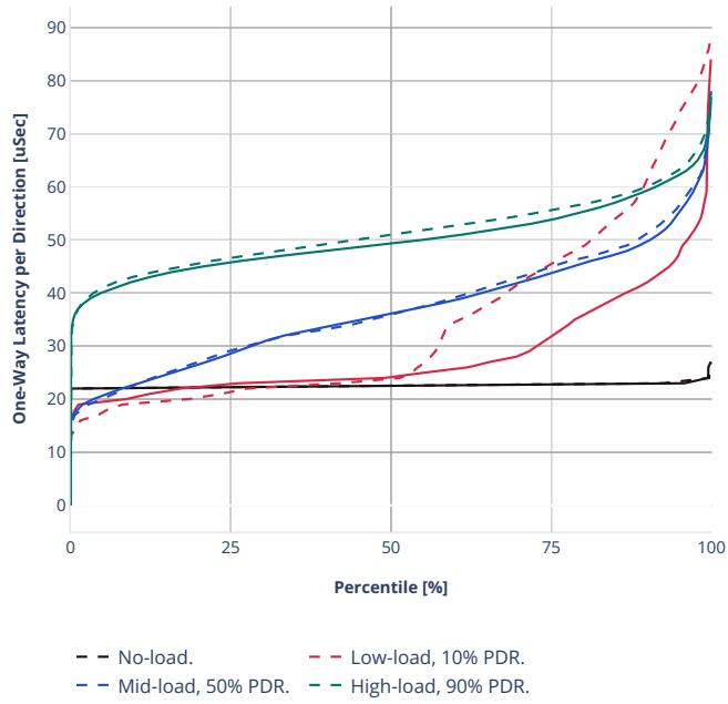
Latency: ethip4-ip4base
