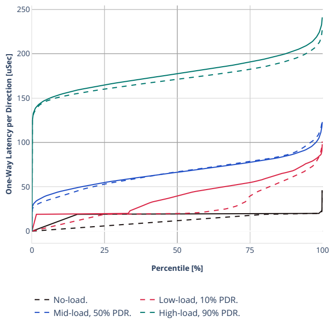
Latency: eth-l2xcbase-eth-2vhostvr1024-1vm
