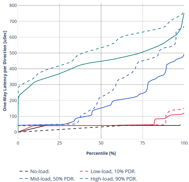
Latency: avf-ethip4ipsec1000tnlsw-ip4base-int-aes128cbc-hmac512sha
