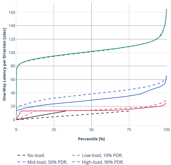
Latency: avf-ethip4-ip4base-eth-2memif-1dcr
