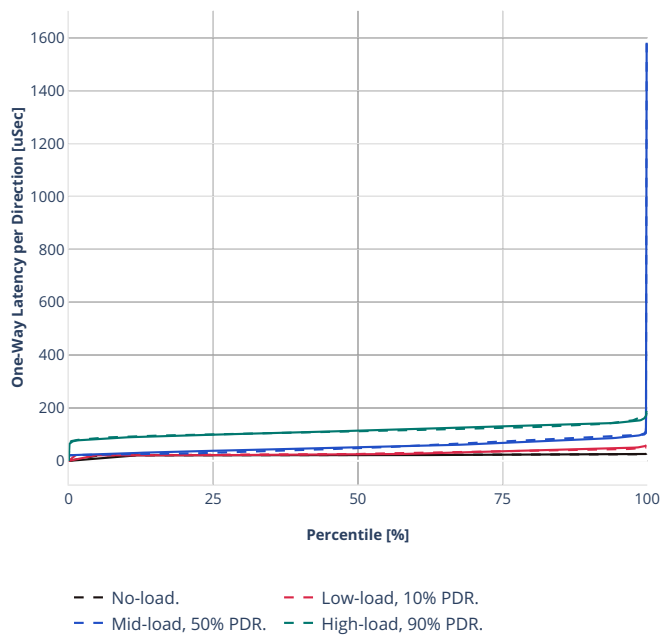
Latency: ethip4-ip4scale2m
