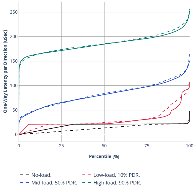
Latency: avf-dot1q-l2bdbasemaclrn-eth-2vhostvr1024-1vm
