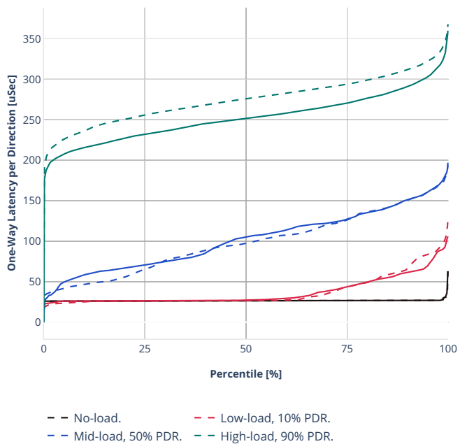
Latency: dot1q-l2bdbasemaclrn-eth-2vhostvr1024-1vm
