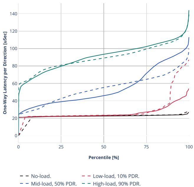
Latency: ethip4udp-ip4base-iac150sl-10kflows
