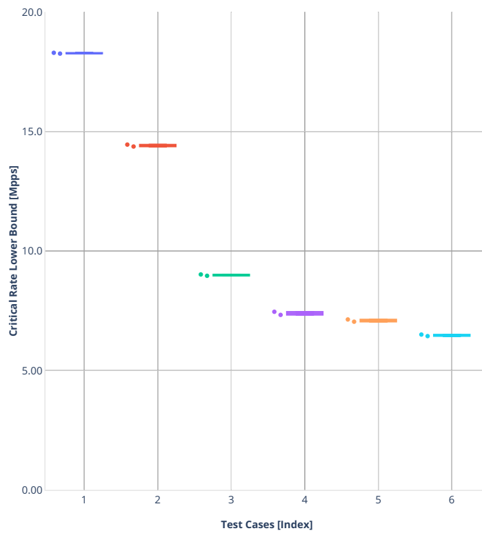
Throughput: 30 Minutes Soak Test (PLRsearch)
