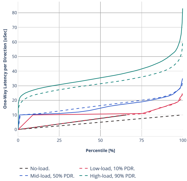
Latency: avf-eth-l2bdscale1mmaclrn
