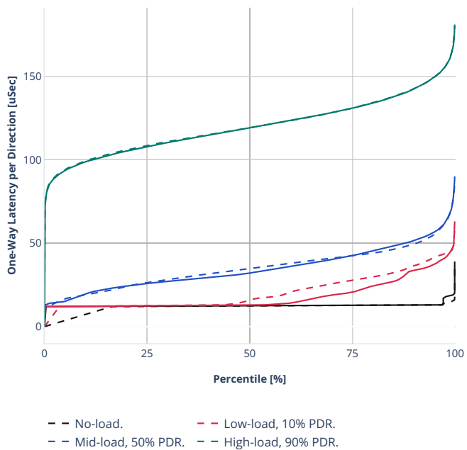
Latency: eth-l2bdbasemaclrn-eth-2vhostvr1024-1vm
