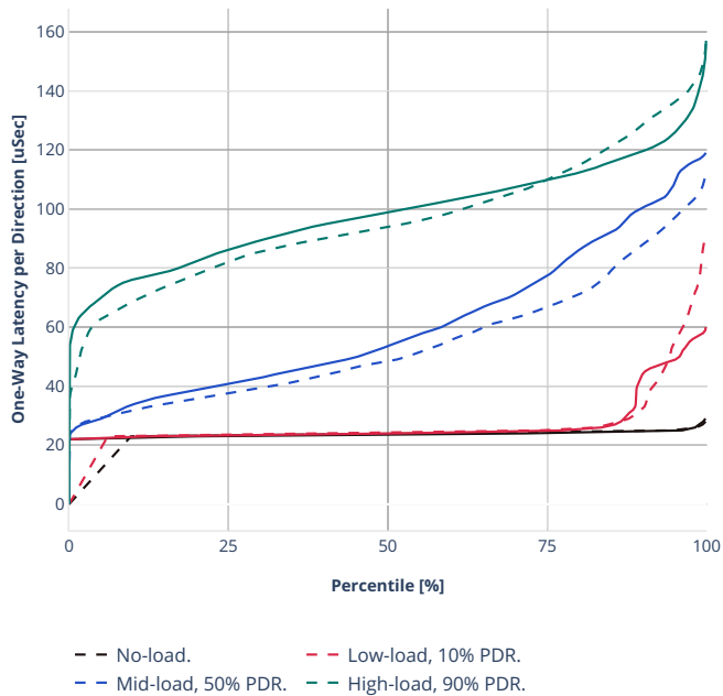
Latency: ethip4udp-ip4base-oac150sl-10kflows
