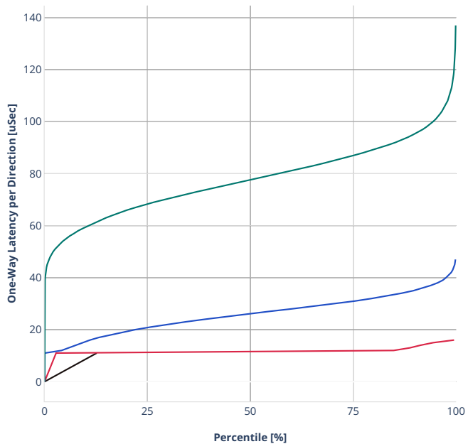
Latency: avf-ethip4udp-nat44ed-h4096-p63-s258048-udir
