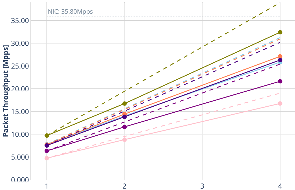
Number of Cores [Qty] --- Perfect — Measured ... Limit avf-dot1q-l2xcbase-eth-2vhostvr1024-1vm avf-eth-l2xcbase-eth-2vhostvr1024-1vm avf-dot1q-l2bdbasemaclrn-eth-2vhostvr1024-1vm avf-eth-l2bdbasemaclrn-eth-2vhostvr1024-1vm avf-ethip4-ip4base-eth-2vhostvr1024-1vm avf-ethip4-vxlan-l2bdbasemaclrn-eth-2vhostvr1024-1vm
