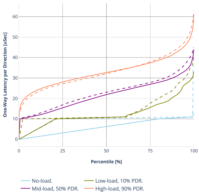
Latency: ethip6-ip6scale200k
