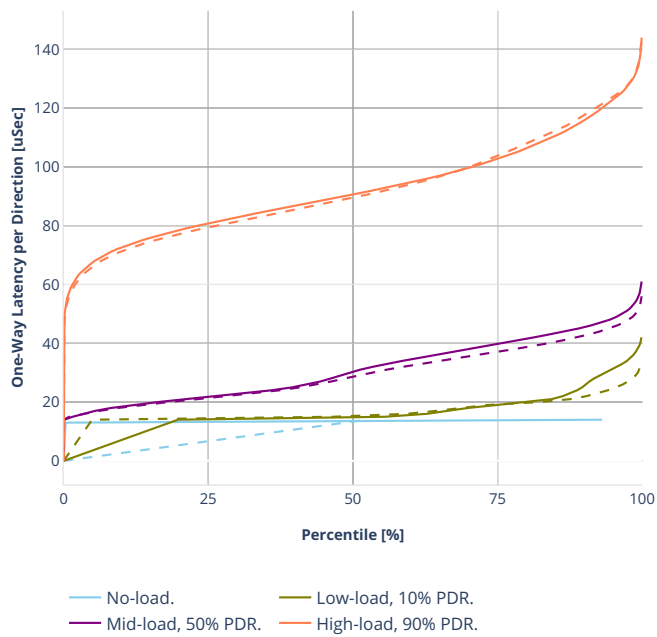
Latency: avf-eth-l2bdbasemaclrn-eth-2memif-1dcr
