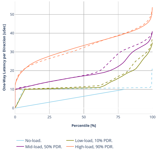
Latency: avf-ethip4-ip4scale2m-rnd
