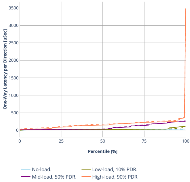
Latency: eth-l2bdbasemaclrn-macip-iac150sl-10kflows
