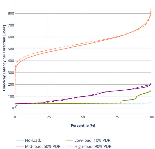
Latency: eth-l2xcbase-eth-2memif-1dcr
