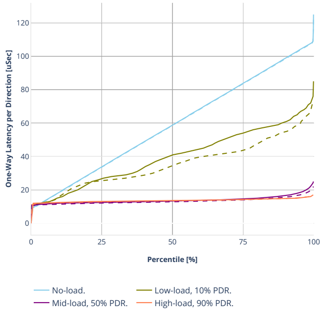
Latency: ethip4-ip4base-l3fwd
