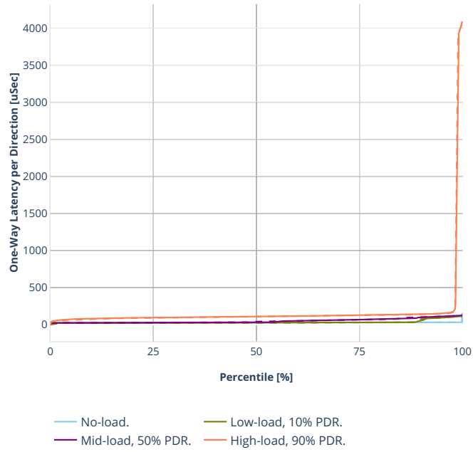
Latency: ethip4-ip4scale200k
