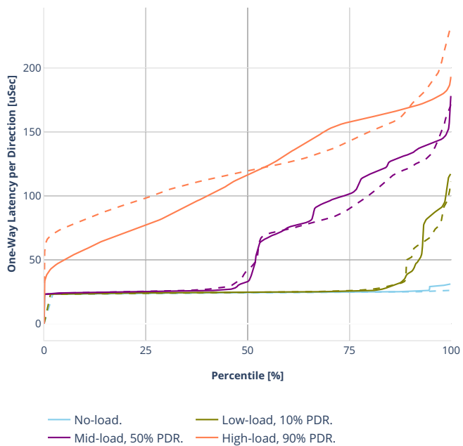
Latency: ethip4udp-ip4base-oac150sl-10kflows
