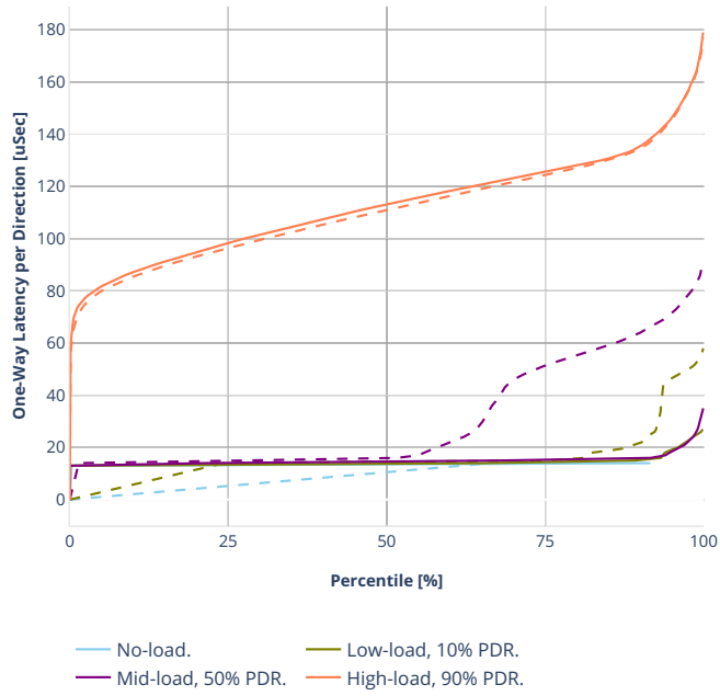
Latency: eth-l2bdbasemaclrn-eth-2memif-1dcr
