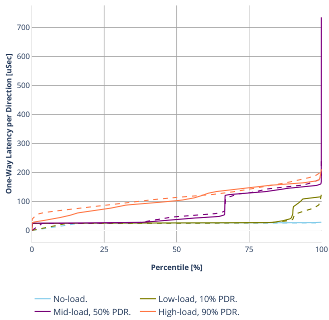
Latency: eth-l2bdbasemaclrn-iac150sl-10kflows
