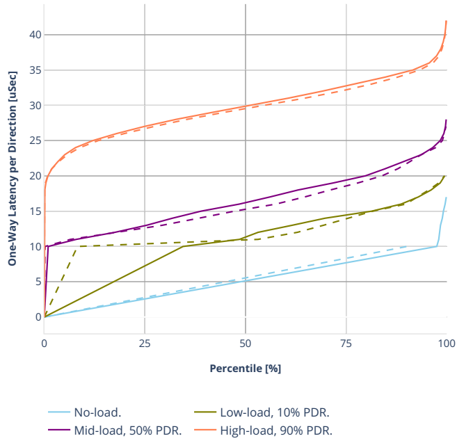
Latency: avf-eth-l2bdscale10kmaclrn
