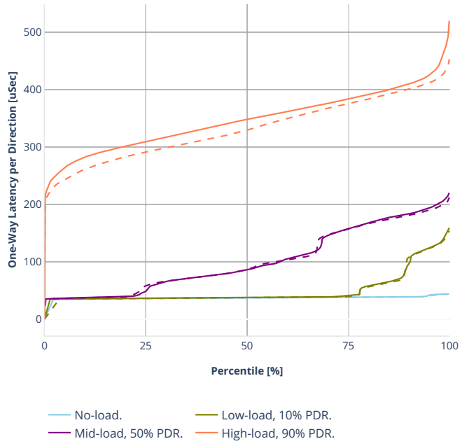
Latency: ethip6srhip6-ip6base-srv6proxy-masq
