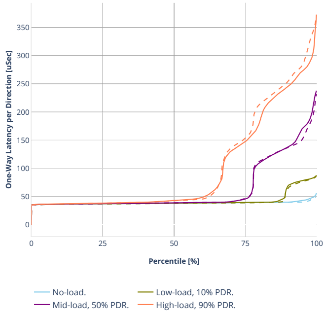
Latency: eth-l2xcbase-eth-2vhostvr1024-1vm-vppl2xc
