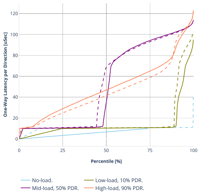
Latency: ethip6-ip6scale2m
