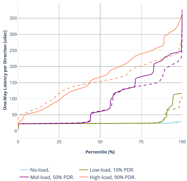
Latency: ethip4udp-ip4base-nat44
