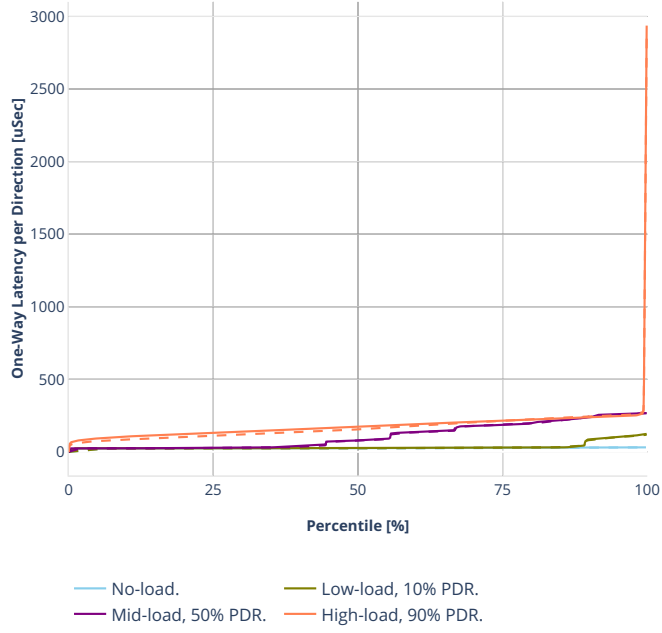
Latency: dot1q-l2bdbasemaclrn
