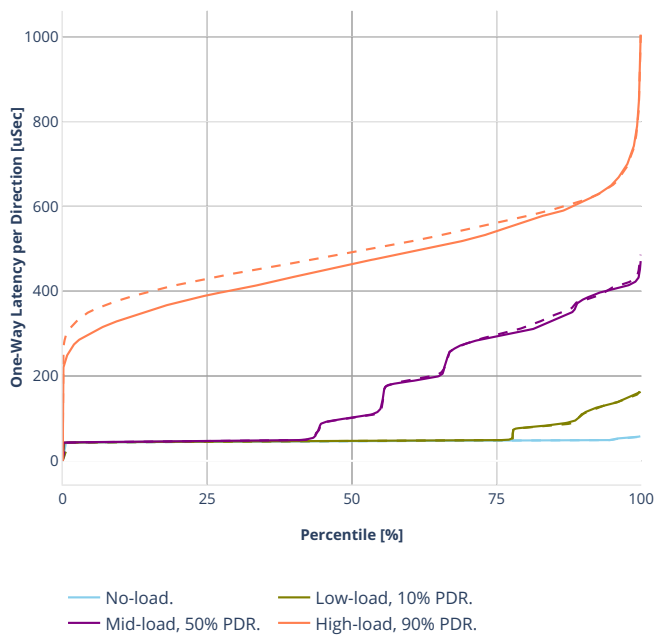
Latency: eth-l2bdbasemaclrn-eth-2memif-1lxc
