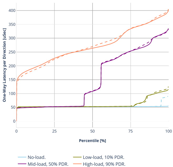
Latency: ethip4ipsec1tnlhw-ip4base-int-aes256gcm
