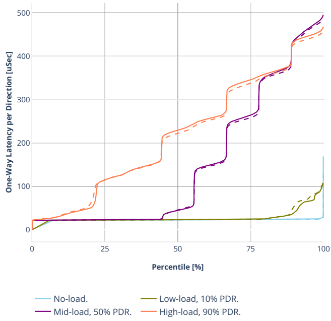
Latency: ethip6-ip6scale200k
