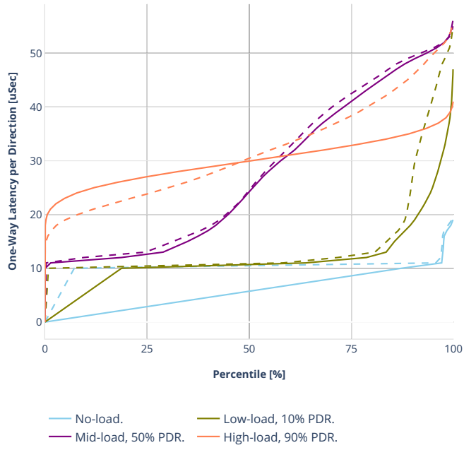
Latency: avf-ethip4-ip4scale20k
