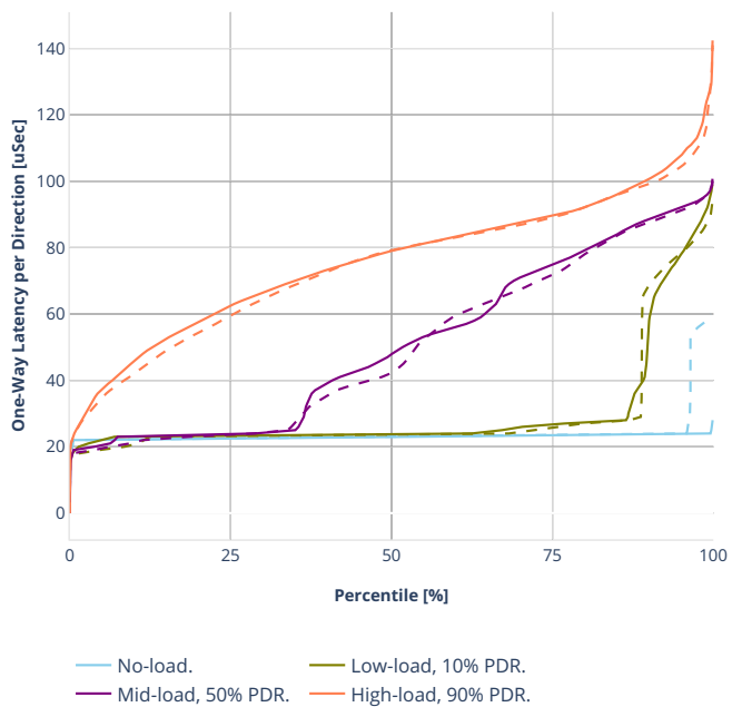
Latency: ethip6-ip6base
