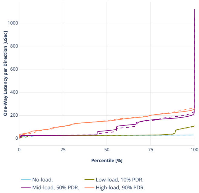
Latency: eth-l2bdscale10kmaclrn
