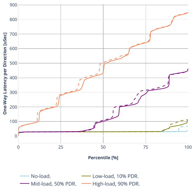
Latency: ethip4ipsec4tnlsw-ip4base-int-aes256gcm
