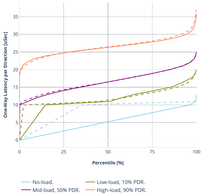
Latency: avf-eth-l2xcbase
