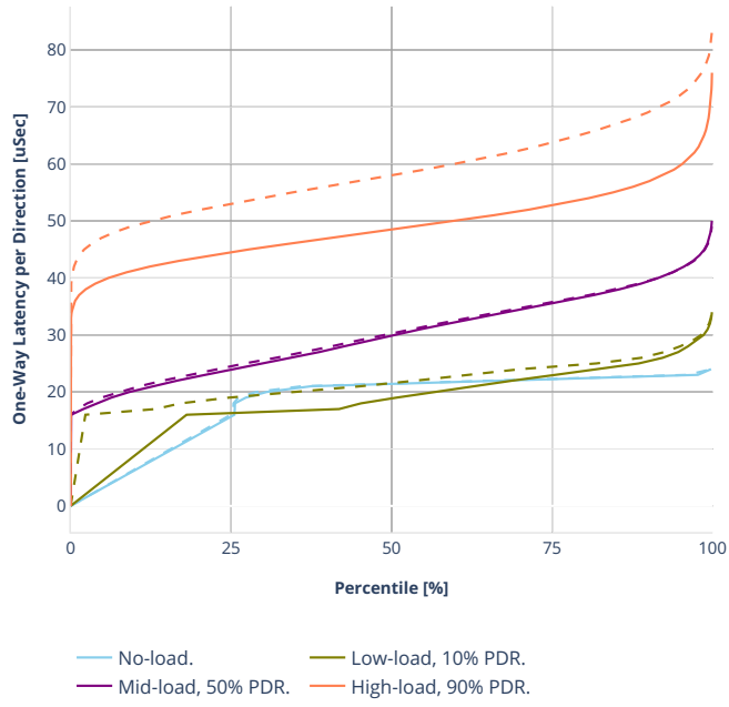
Latency: avf-ethip4-ip4scale200k
