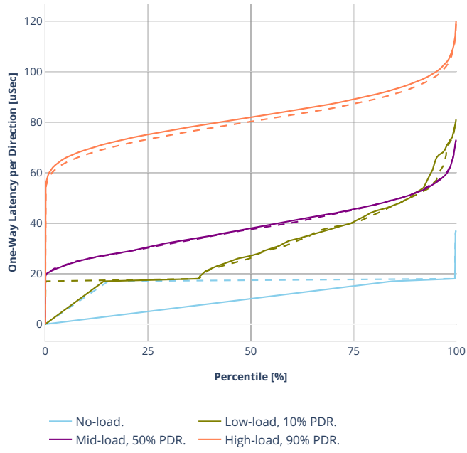
Latency: ethip4vxlan-l2bdbasemaclrn
