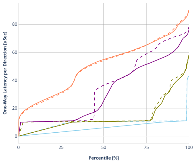
Latency: ethip6-ip6scale20k
