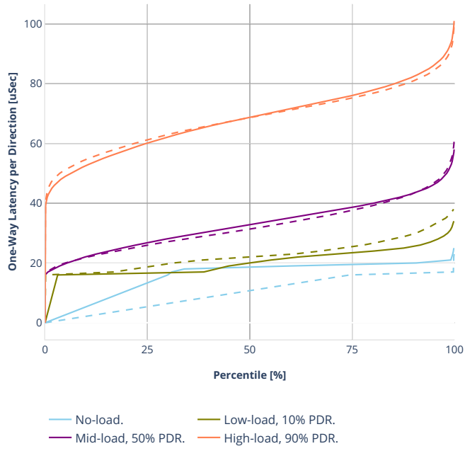
Latency: avf-eth-l2bdscale100kmac1rn
