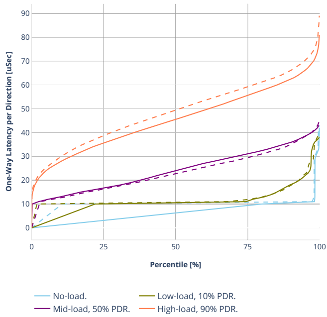
Latency: eth-l2bdscale100kmacirn
