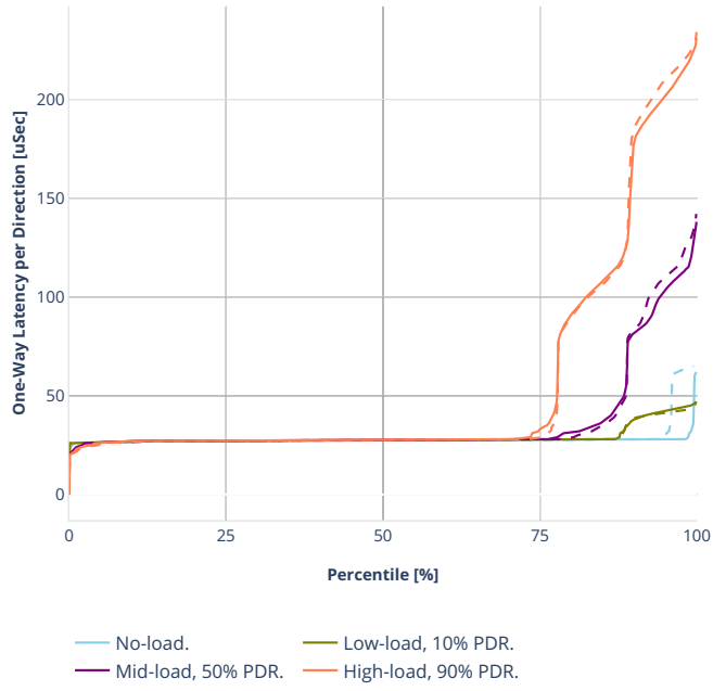
Latency: dot1q-l2xcbase-eth-2vhostvr1024-1vm-vppl2xc
