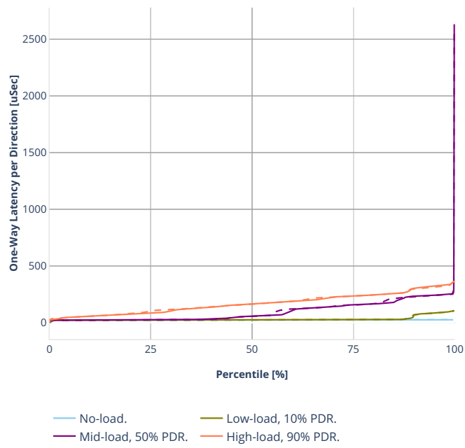
Latency: ethip4-ip4scale200k
