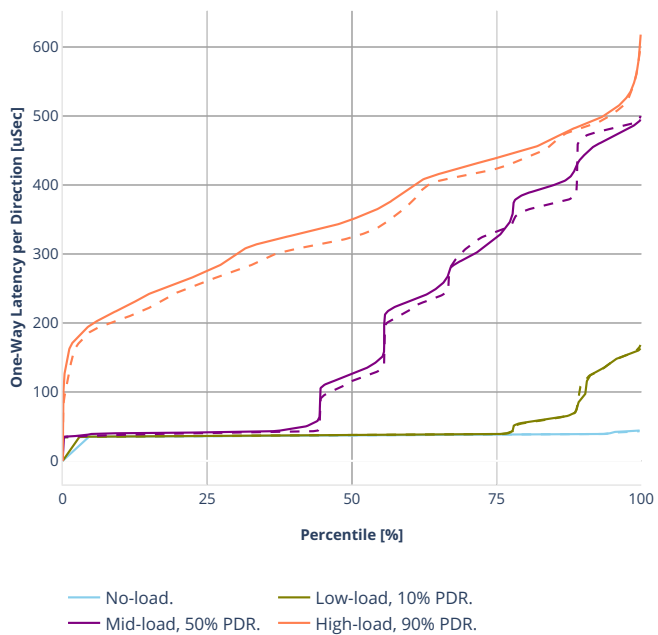
Latency: ethip6srhip6-ip6base-srv6proxy-masq
