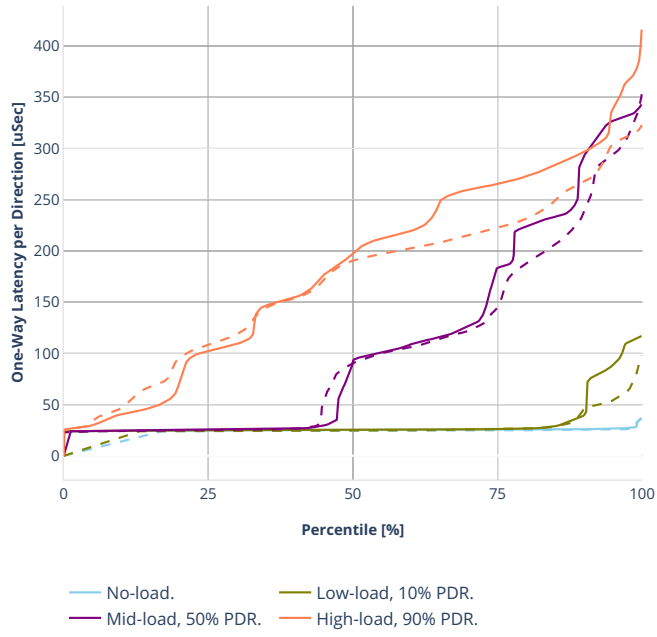
Latency: eth-l2bdbasemaclrn-iac150sl-10kflows
