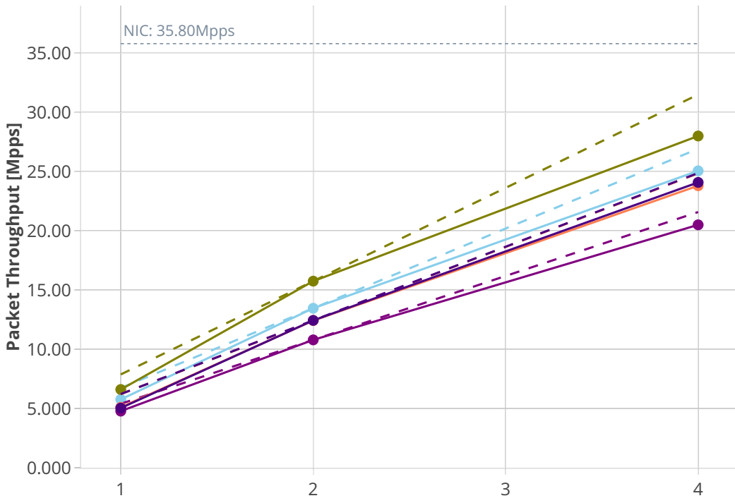
- - Perfect — Measred ... Limit ● dot1q-l2xcbase-eth-2vhostvr1024-1vm-vppl2xc ● eth-l2xcbase-eth-2vhostvr1024-1vm-vppl2xc ● dot1q-l2bdbasemaclrn-eth-2vhostvr1024-1vm-vppl2xc ● eth-l2bdbasemaclrn-eth-2vhostvr1024-1vm-vppl2xc ● ethip4-ip4base-eth-2vhostvr1024-1vm-vppip4
