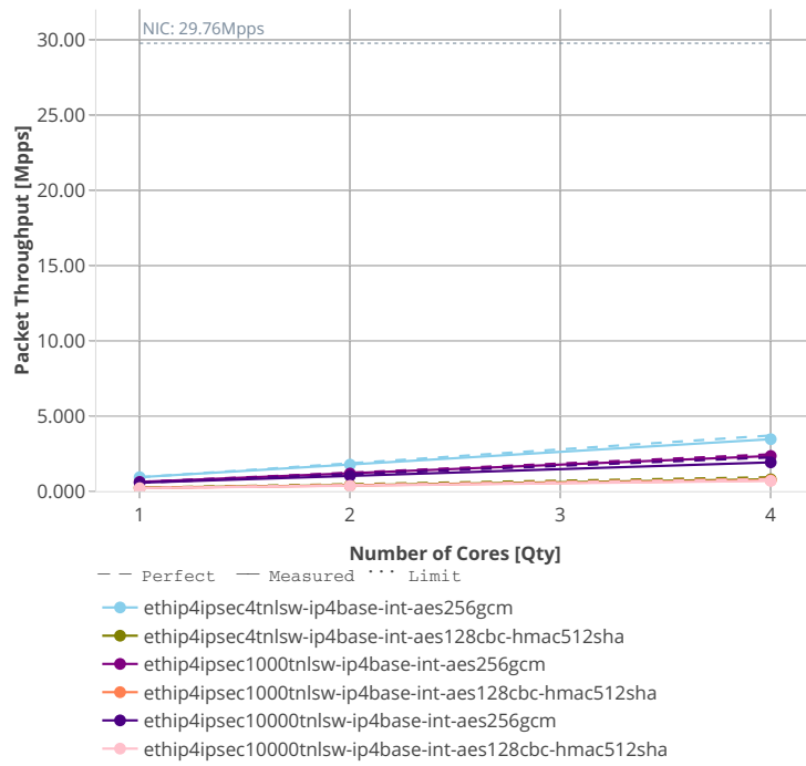
Speedup Multi-core: 3n-dnv-x553-imix-ipsec-ip4routing-base-scale-sw-ixgbe
