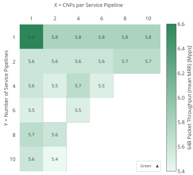
Throughput: eth-l2bd-{Y}pl-{2Y}mif-{XY}dcr-vppip4-mrr
