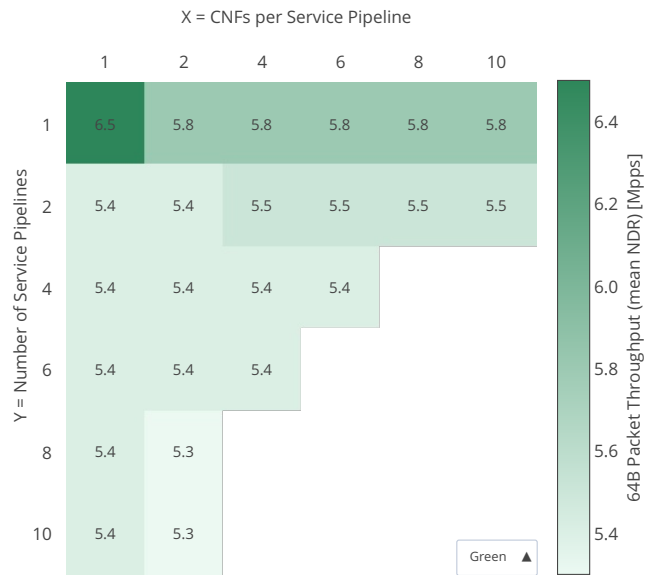
Throughput: eth-l2bd-{Y}pl-{2Y}mif-{XY}dcr-vppip4-ndr
