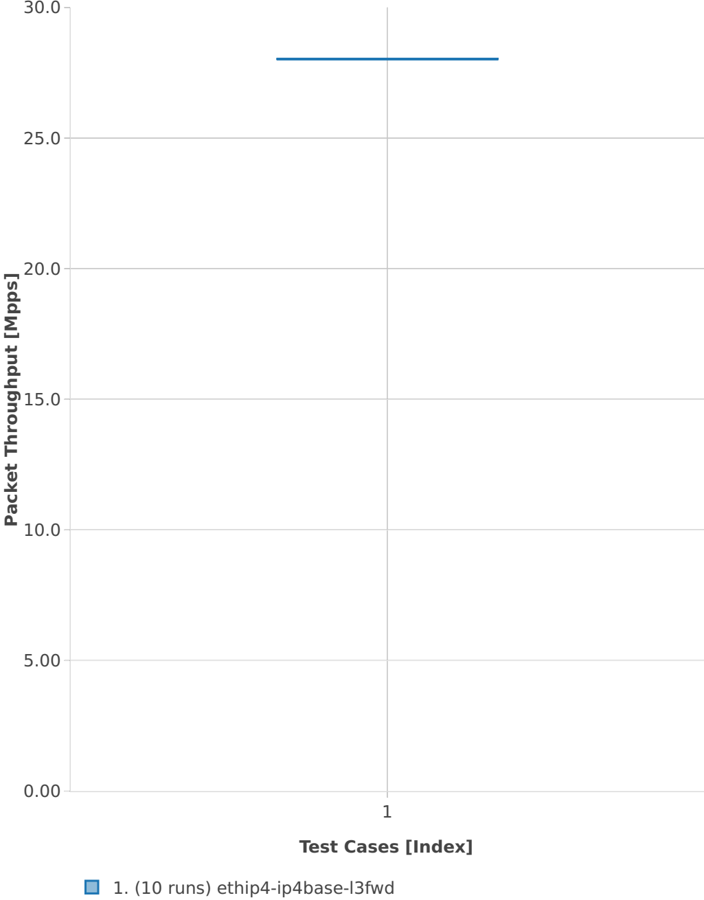
Throughput: l3fwd-3n-skx-x710-64b-2t1c-base-pdr
