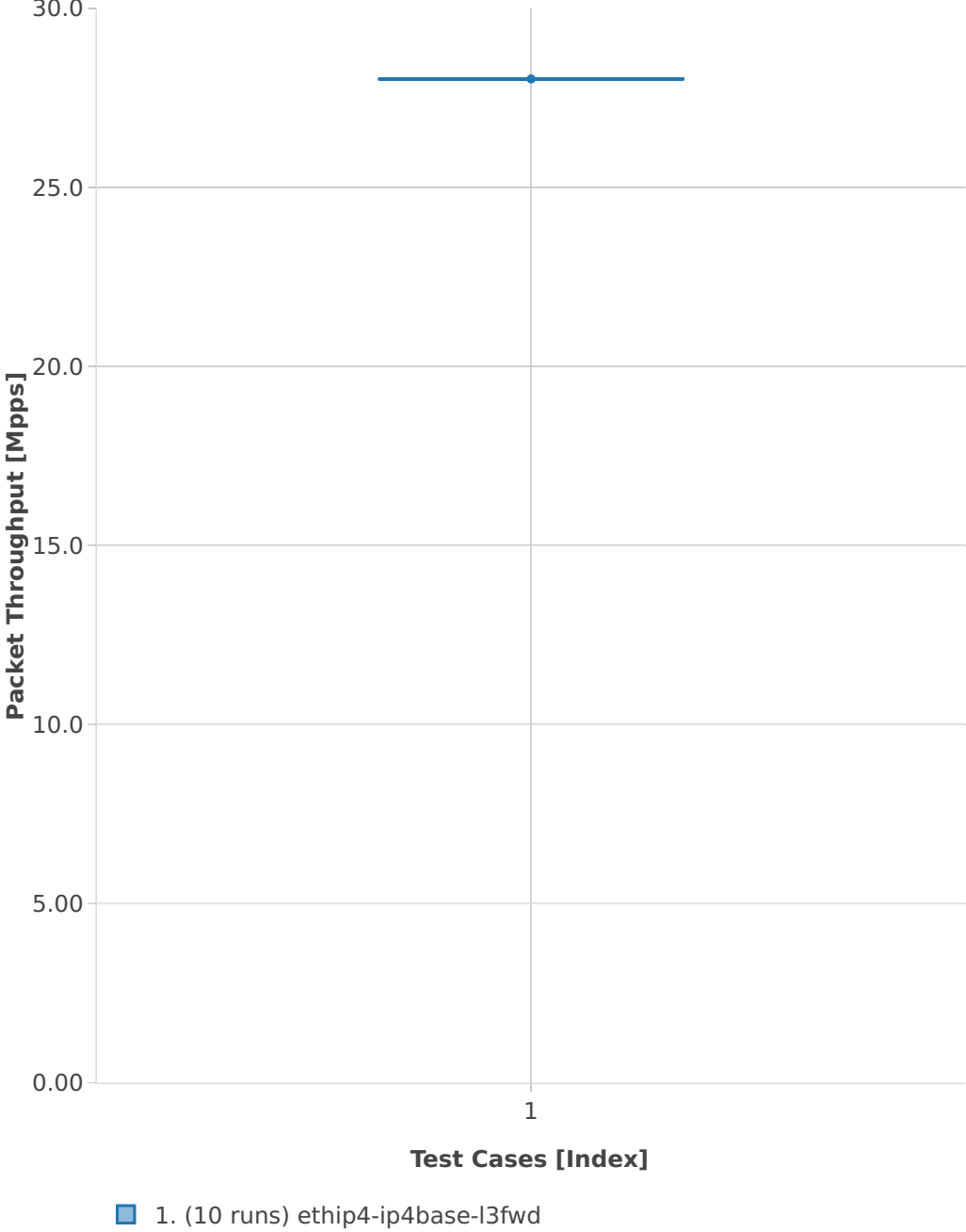
Throughput: l3fwd-2n-skx-x710-64b-2t1c-base-pdr
