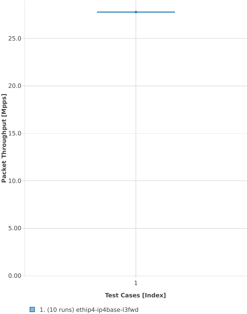
Throughput: l3fwd-2n-skx-x710-64b-2t1c-base-ndr
