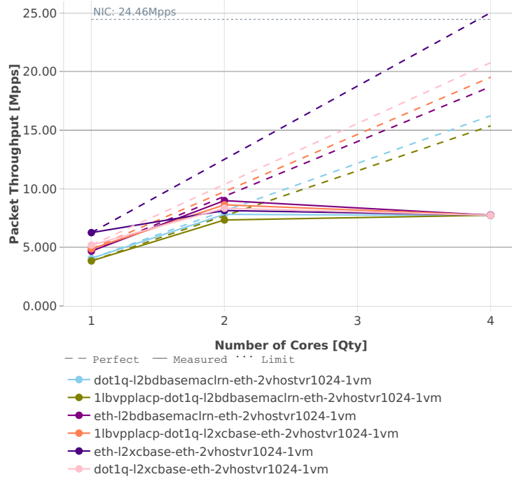
Speedup Multi-core: vhost-l2sw-3n-hsw-x520-64b-base_and_features-pdr
