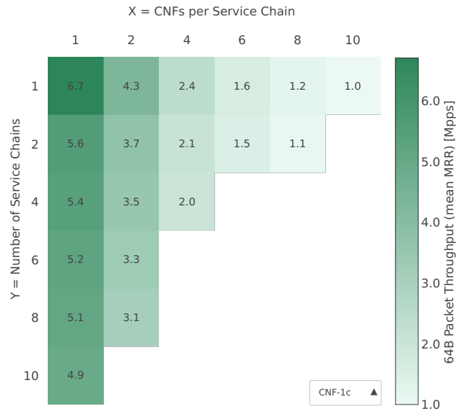
Throughput: eth-l2bd-{Y}ch-{2XY}mif-{XY}dcr-vppip4-mrr
