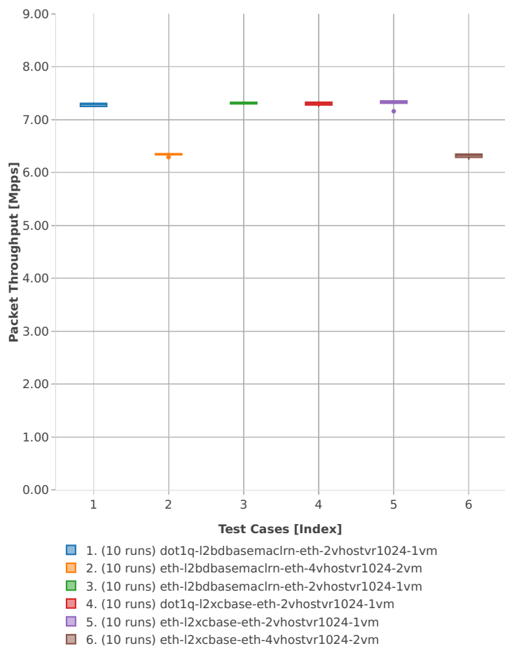
Throughput: vhost-l2sw-3n-skx-x710-64b-4t2c-base_and_features-vm-pdr
