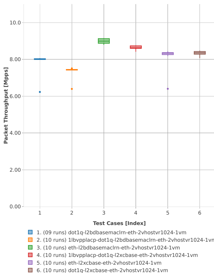
Throughput: vhost-l2sw-3n-hsw-x520-64b-2t2c-base_and_features-pdr
