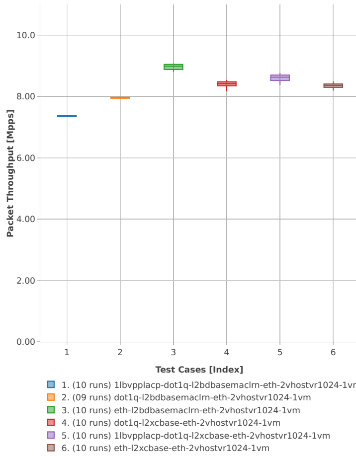
Throughput: vhost-l2sw-3n-hsw-x710-64b-2t2c-base_and_features-pdr
