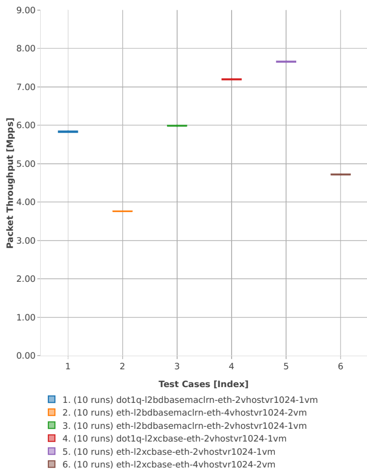
Throughput: vhost-l2sw-3n-skx-x710-64b-2t1c-base_and_features-vm-pdr
