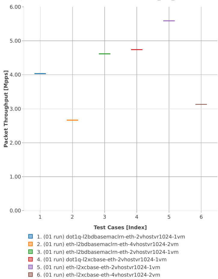
Throughput: vhost-l2sw-3n-hsw-x710-64b-1t1c-base_and_features-vm-pdr
