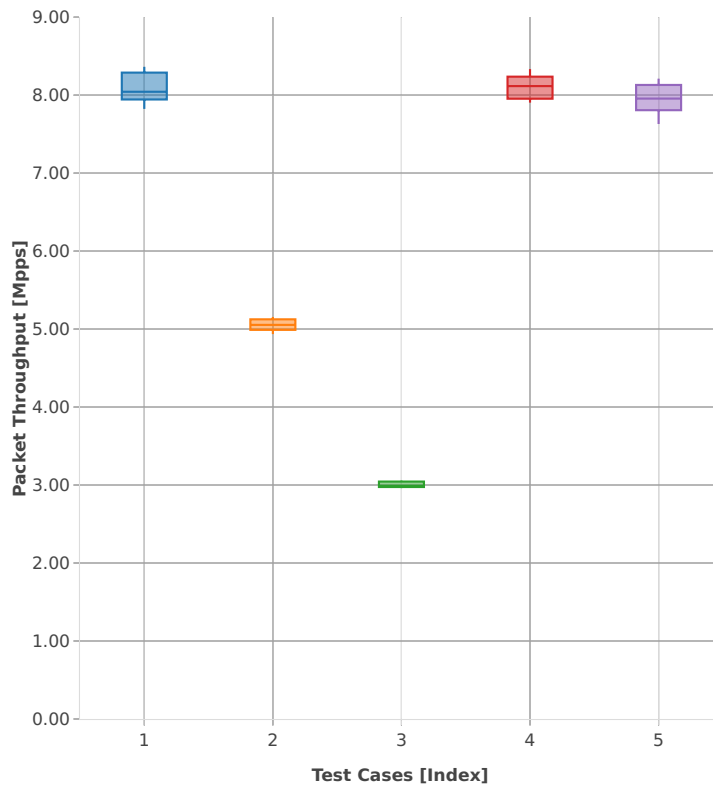
Throughput: k8s-memif-3n-hsw-x710-64b-2t2c-base_and_scale-l2bd-ndr
