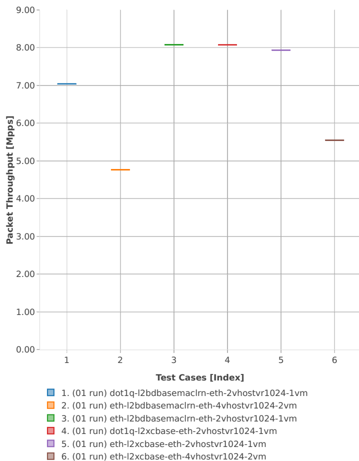
Throughput: vhost-l2sw-3n-hsw-x710-64b-2t2c-base_and_features-vm-pdr
