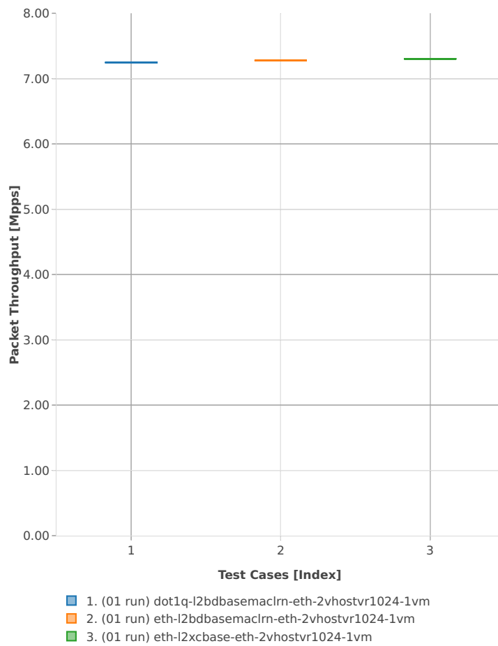
Throughput: vhost-l2sw-2n-skx-xxv710-64b-4t2c-base_and_features-ndr
