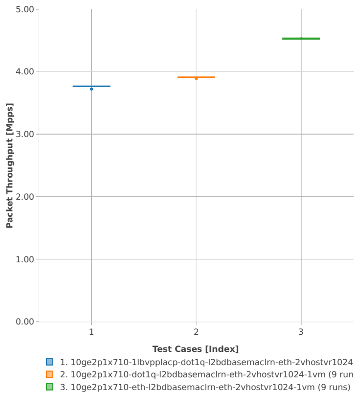
Packet Throughput: vhost-l2sw-3n-hsw-x710-64b-1t1c-base_and_scale-pdr
