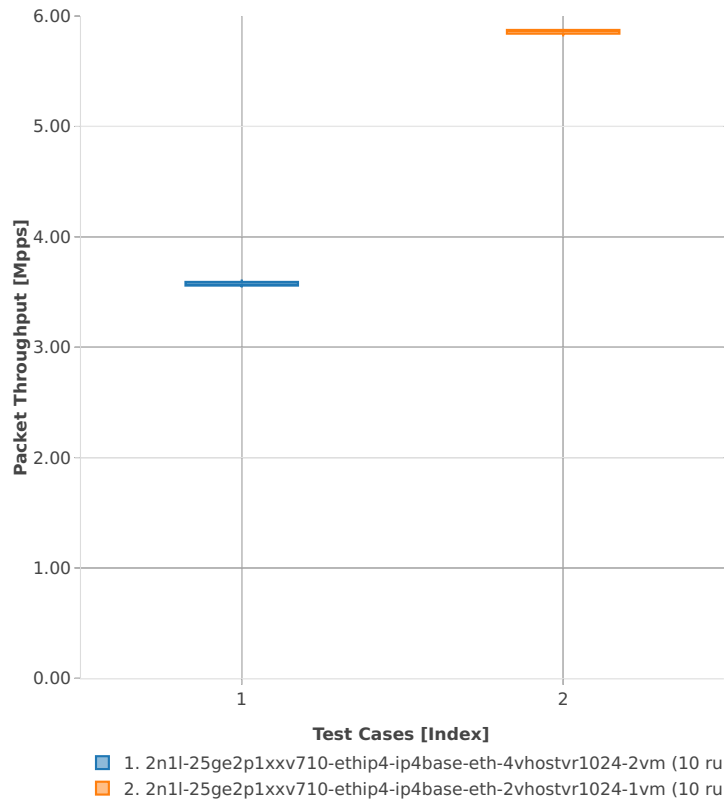
Packet Throughput: vhost-ip4-2n-skx-xxv710-64b-2t1c-base_and_scale-ndr
