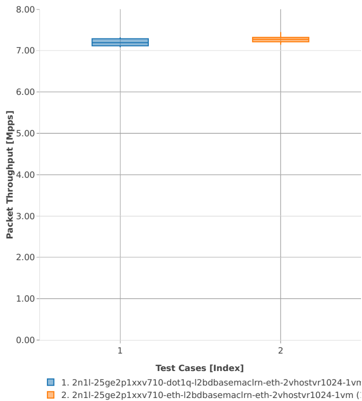
Packet Throughput: vhost-l2sw-2n-skx-xxv710-64b-4t2c-base_and_scale-pd
