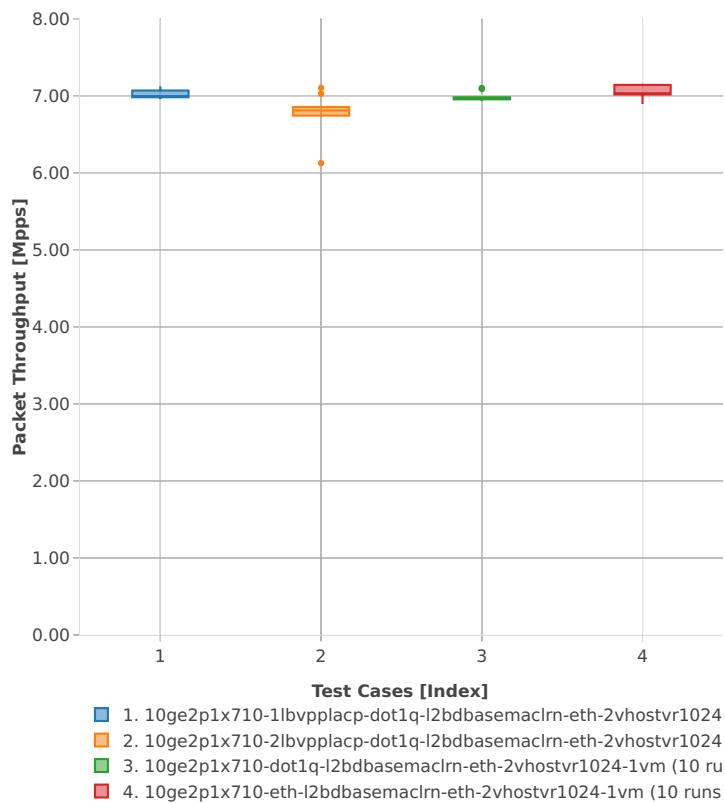
Packet Throughput: vhost-l2sw-3n-skx-x710-64b-4t2c-base_and_scale-pdr
