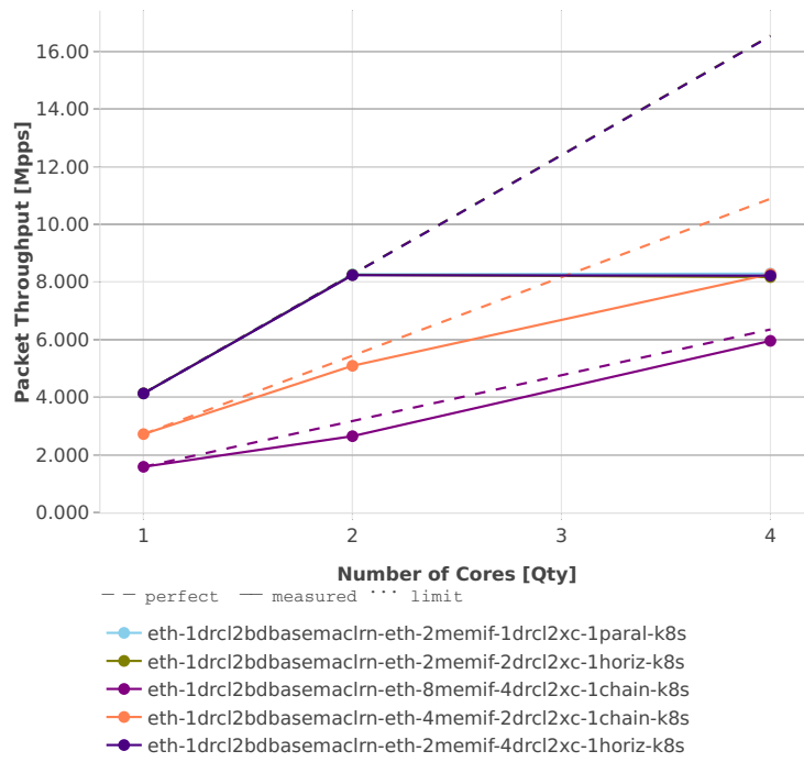
Speedup Multi-core: k8s-memif-3n-hsw-x520-64b-base_and_scale-l2bd-pdr
