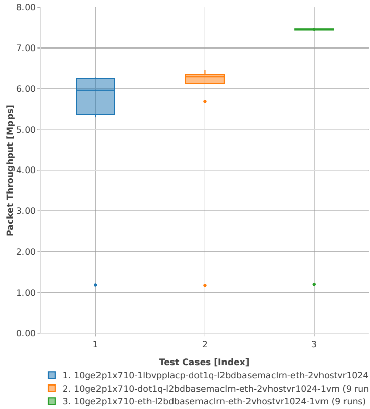
Packet Throughput: vhost-l2sw-3n-hsw-x710-64b-2t2c-base_and_scale-ndr
