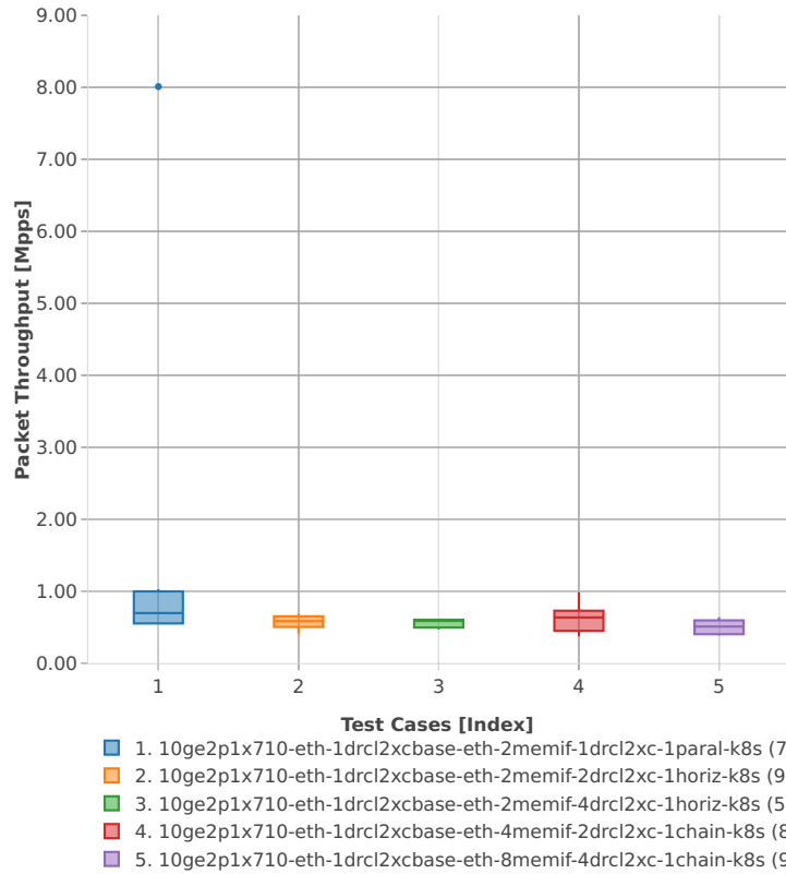
Packet Throughput: k8s-memif-3n-hsw-x710-64b-2t2c-base_and_scale-l2xc-n
