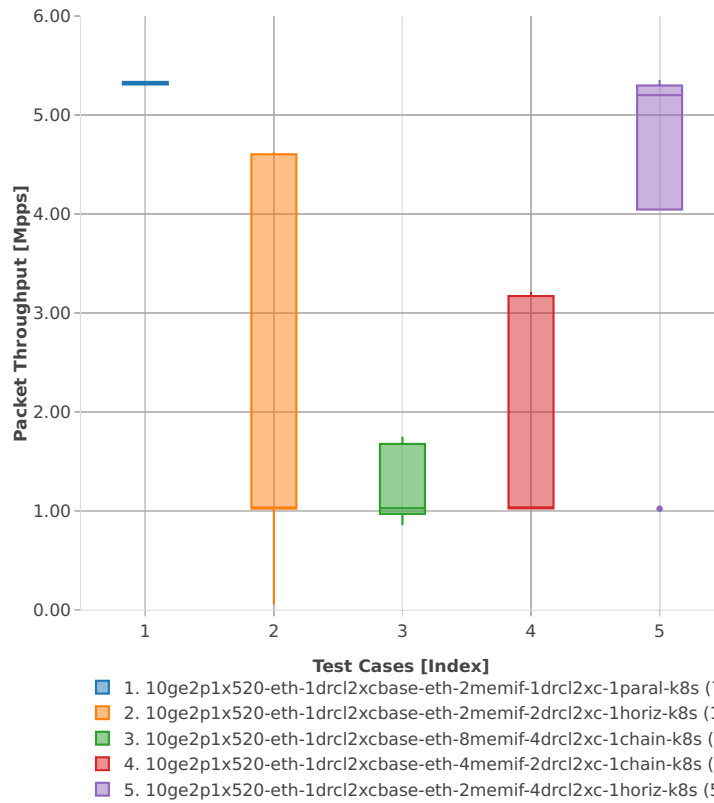
Packet Throughput: k8s-memif-3n-hsw-x520-64b-1t1c-base_and_scale-l2xc-n
