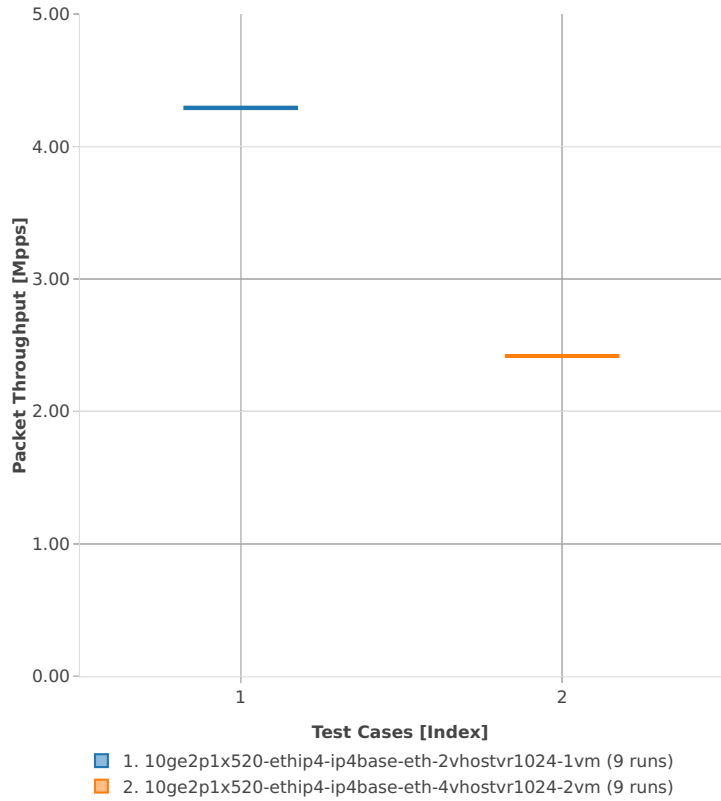
Packet Throughput: vhost-ip4-3n-hsw-x520-64b-1t1c-base_and_scale-ndr
