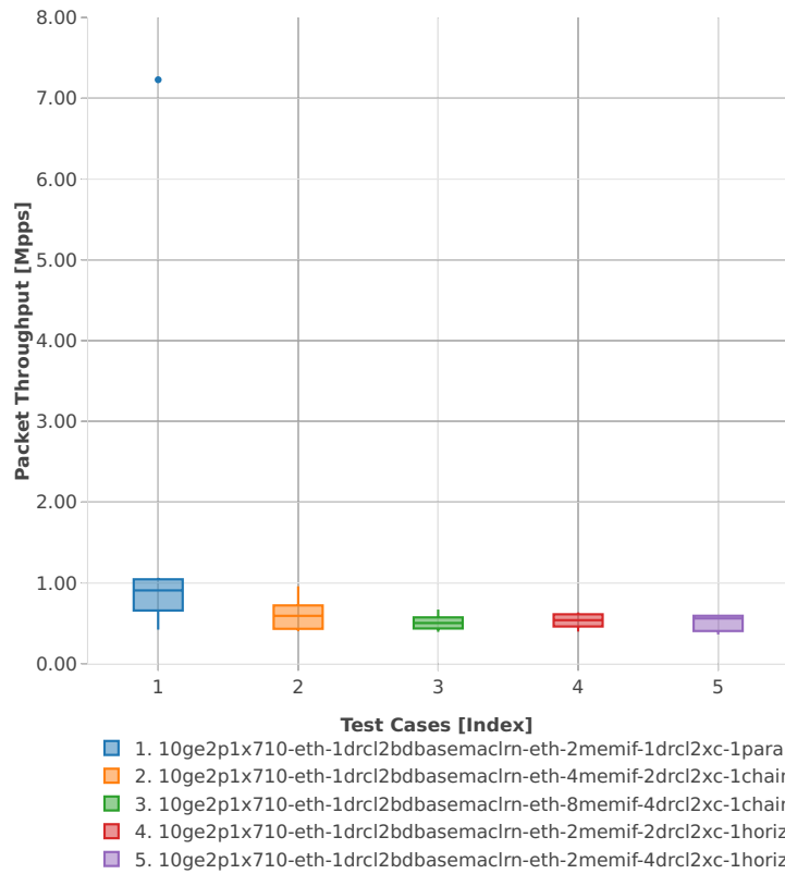
Packet Throughput: k8s-memif-3n-hsw-x710-64b-2t2c-base_and_scale-l2bd-n
