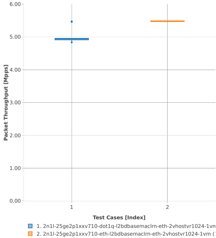
Packet Throughput: vhost-l2sw-2n-skx-xxv710-64b-2t1c-base_and_scale-nd
