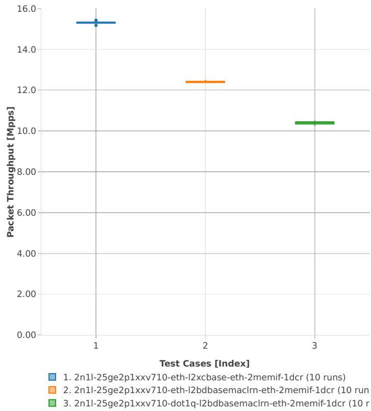
Packet Throughput: memif-2n-skx-xxv710-64b-4t2c-base_and_scale-pdr
