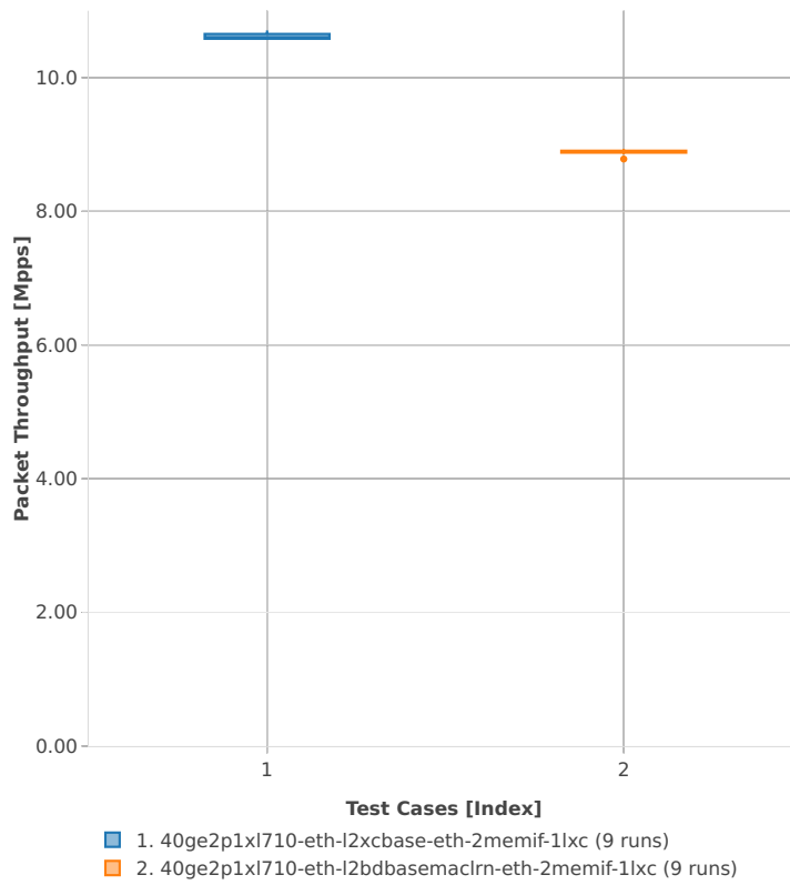
Packet Throughput: memif-3n-hsw-xl710-64b-2t2c-base_and_scale-pdr
