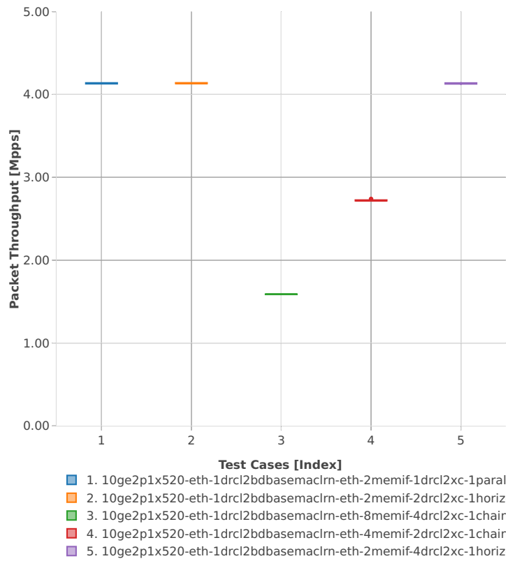
Packet Throughput: k8s-memif-3n-hsw-x520-64b-1t1c-base_and_scale-l2bd-p
