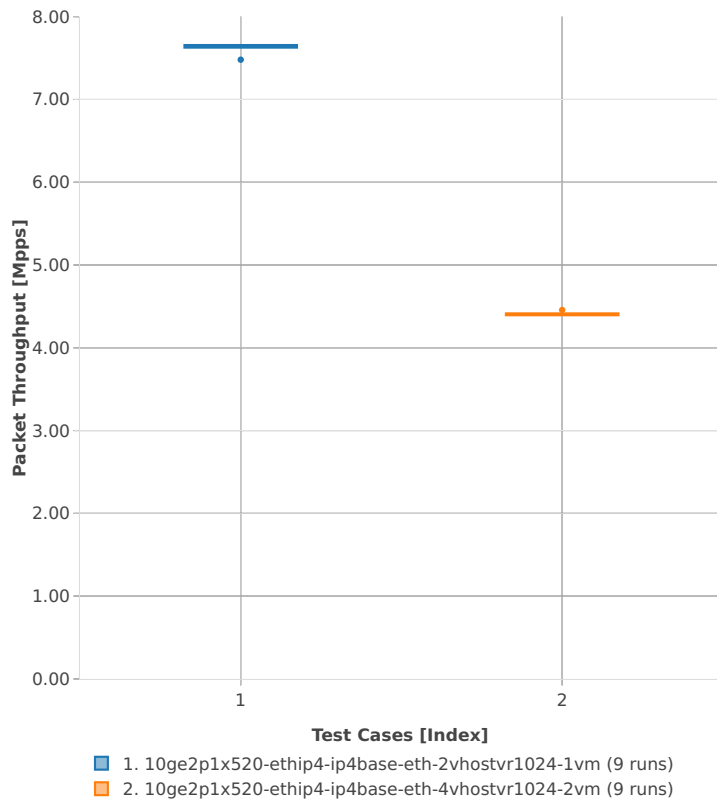
Packet Throughput: vhost-ip4-3n-hsw-x520-64b-2t2c-base_and_scale-pdr
