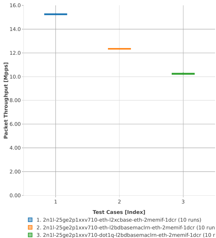
Packet Throughput: memif-2n-skx-xxv710-64b-4t2c-base_and_scale-ndr
