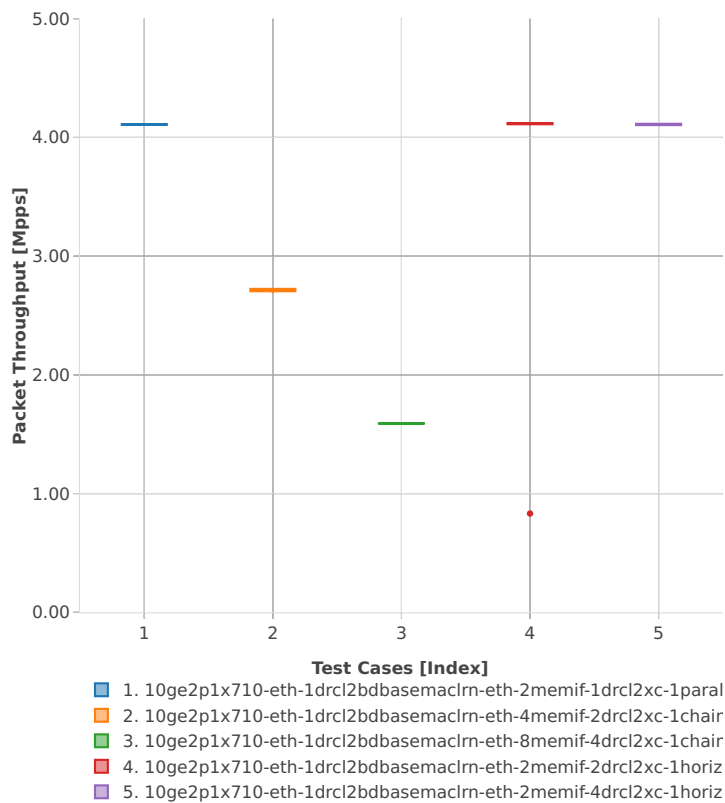
Packet Throughput: k8s-memif-3n-hsw-x710-64b-1t1c-base_and_scale-l2bd-p
