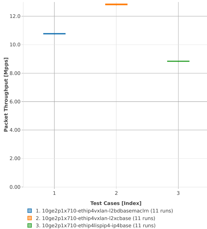
Packet Throughput: ip4tun-3n-skx-x710-64b-2t1c-base_and_features-ndr
