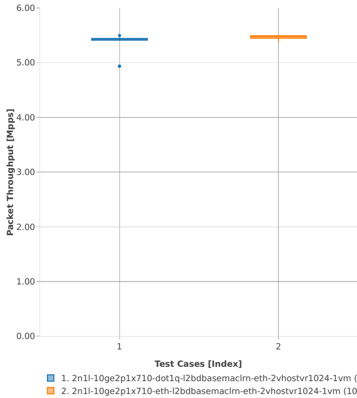
Packet Throughput: vhost-l2sw-2n-skx-x710-64b-2t1c-base_and_scale-ndr
