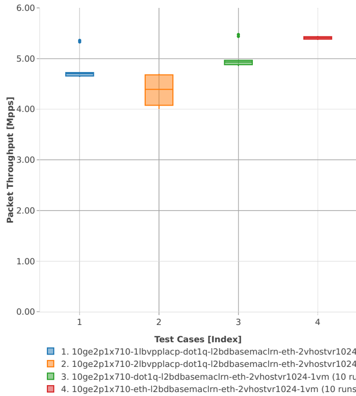
Packet Throughput: vhost-l2sw-3n-skx-x710-64b-2t1c-base_and_scale-ndr
