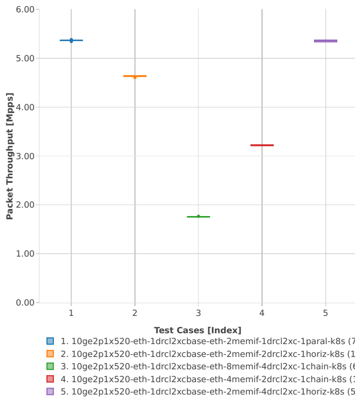
Packet Throughput: k8s-memif-3n-hsw-x520-64b-1t1c-base_and_scale-l2xc-p
