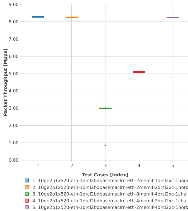
Packet Throughput: k8s-memif-3n-hsw-x520-64b-2t2c-base_and_scale-l2bd-p
