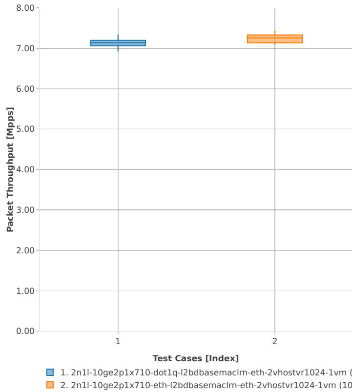
Packet Throughput: vhost-l2sw-2n-skx-x710-64b-4t2c-base_and_scale-ndr
