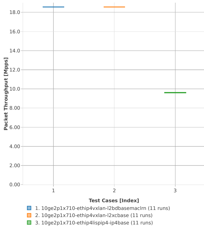
Packet Throughput: ip4tun-3n-skx-x710-64b-4t2c-base_and_features-pdr
