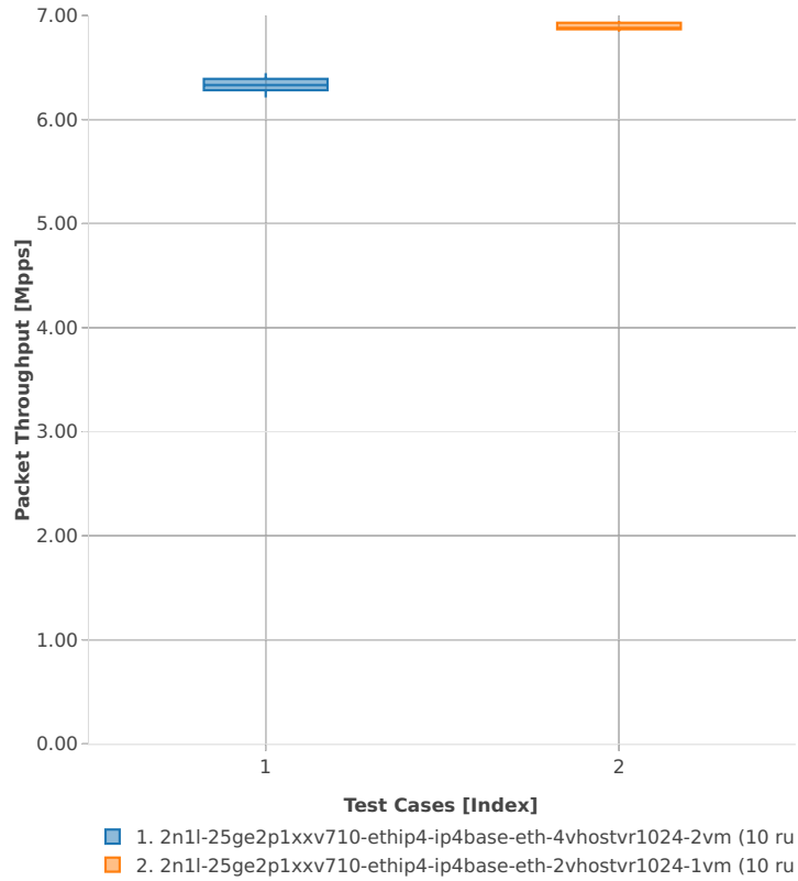
Packet Throughput: vhost-ip4-2n-skx-xxv710-64b-4t2c-base_and_scale-ndr
