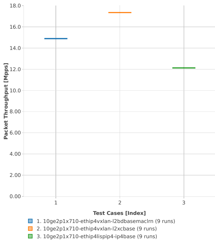
Packet Throughput: ip4tun-3n-hsw-x710-64b-2t2c-base_and_features-pdr
