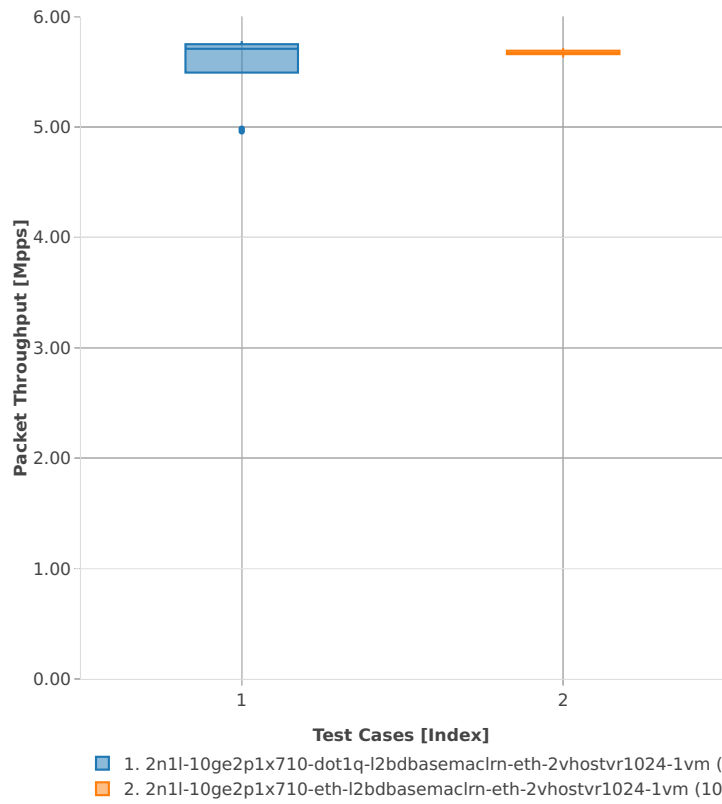
Packet Throughput: vhost-l2sw-2n-skx-x710-64b-2t1c-base_and_scale-pdr
