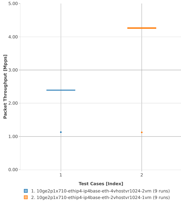
Packet Throughput: vhost-ip4-3n-hsw-x710-64b-1t1c-base_and_scale-ndr
