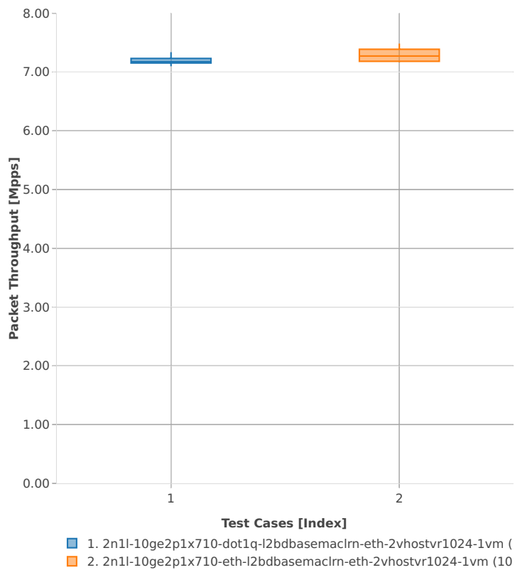
Packet Throughput: vhost-l2sw-2n-skx-x710-64b-4t2c-base_and_scale-pdr
