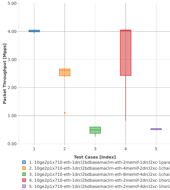
Packet Throughput: k8s-memif-3n-hsw-x710-64b-1t1c-base_and_scale-l2bd-n
