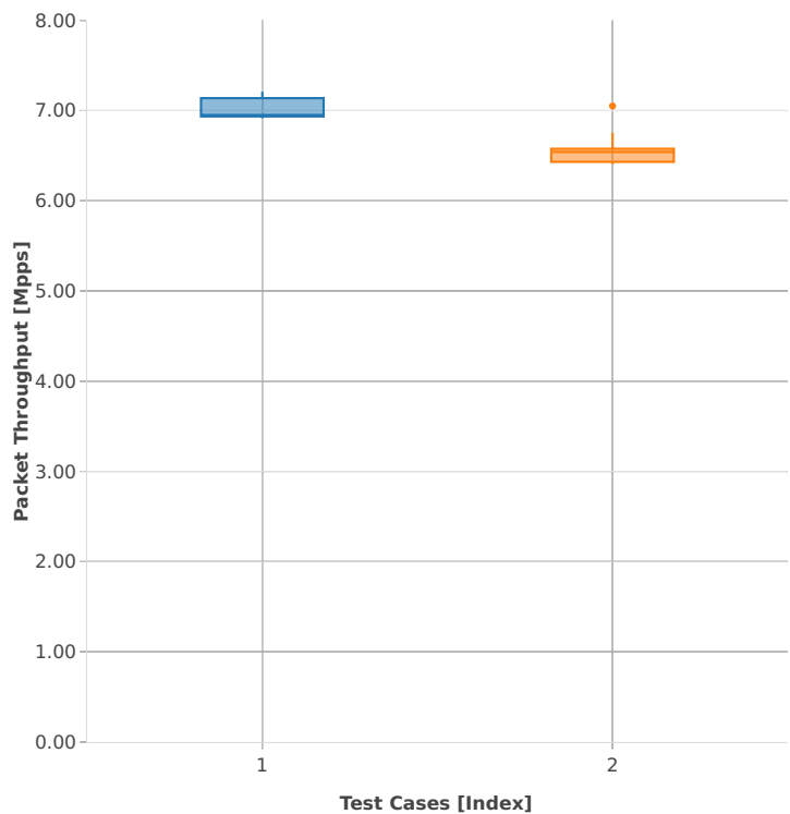
Packet Throughput: vhost-ip4-2n-skx-x710-64b-4t2c-base_and_scale-pdr
