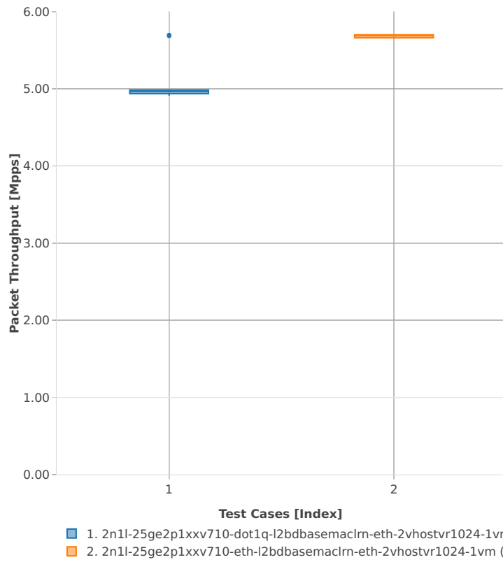
Packet Throughput: vhost-l2sw-2n-skx-xxv710-64b-2t1c-base_and_scale-pd
