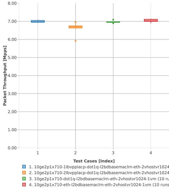
Packet Throughput: vhost-l2sw-3n-skx-x710-64b-4t2c-base_and_scale-ndr
