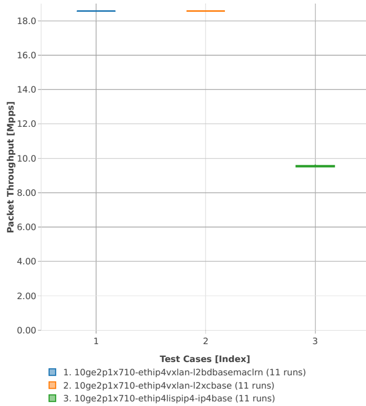
Packet Throughput: ip4tun-3n-skx-x710-64b-4t2c-base_and_features-ndr
