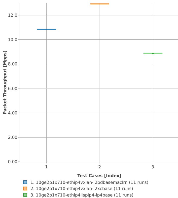
Packet Throughput: ip4tun-3n-skx-x710-64b-2t1c-base_and_features-pdr
