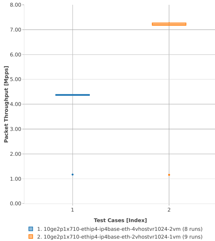
Packet Throughput: vhost-ip4-3n-hsw-x710-64b-2t2c-base_and_scale-ndr
