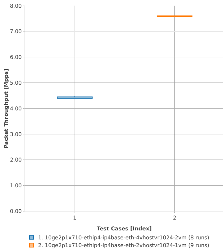
Packet Throughput: vhost-ip4-3n-hsw-x710-64b-2t2c-base_and_scale-pdr
