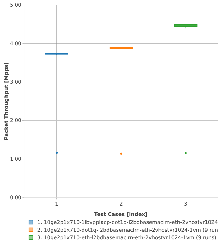
Packet Throughput: vhost-l2sw-3n-hsw-x710-64b-1t1c-base_and_scale-ndr
