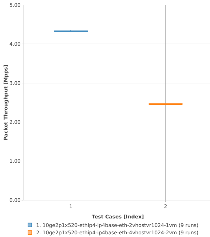
Packet Throughput: vhost-ip4-3n-hsw-x520-64b-1t1c-base_and_scale-pdr
