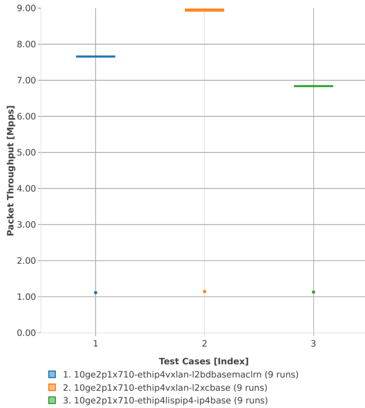
Packet Throughput: ip4tun-3n-hsw-x710-64b-1t1c-base_and_features-ndr
