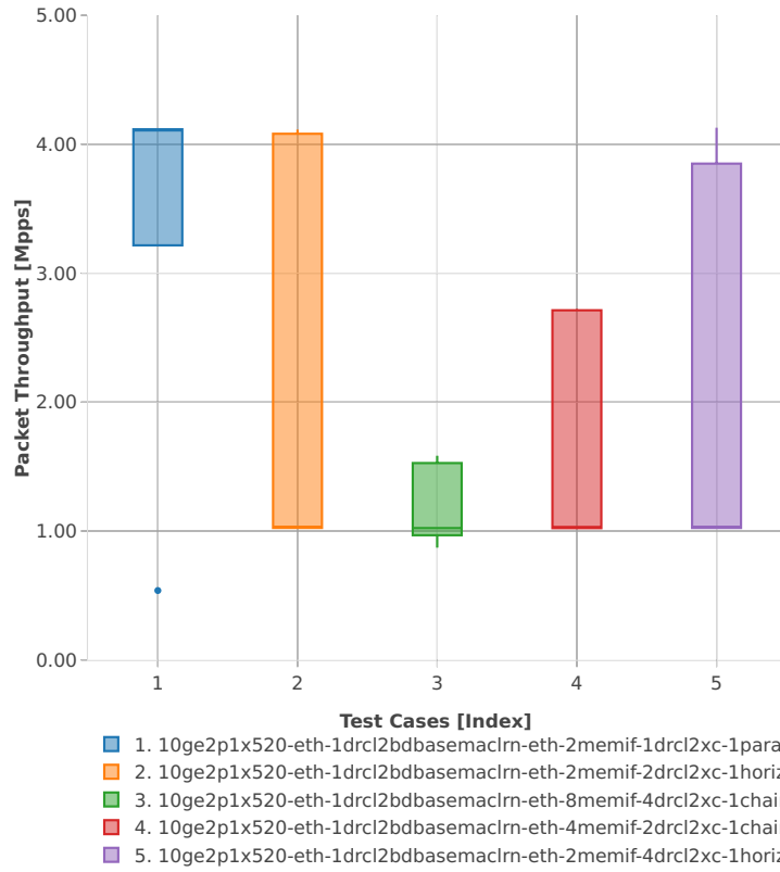
Packet Throughput: k8s-memif-3n-hsw-x520-64b-1t1c-base_and_scale-l2bd-n
