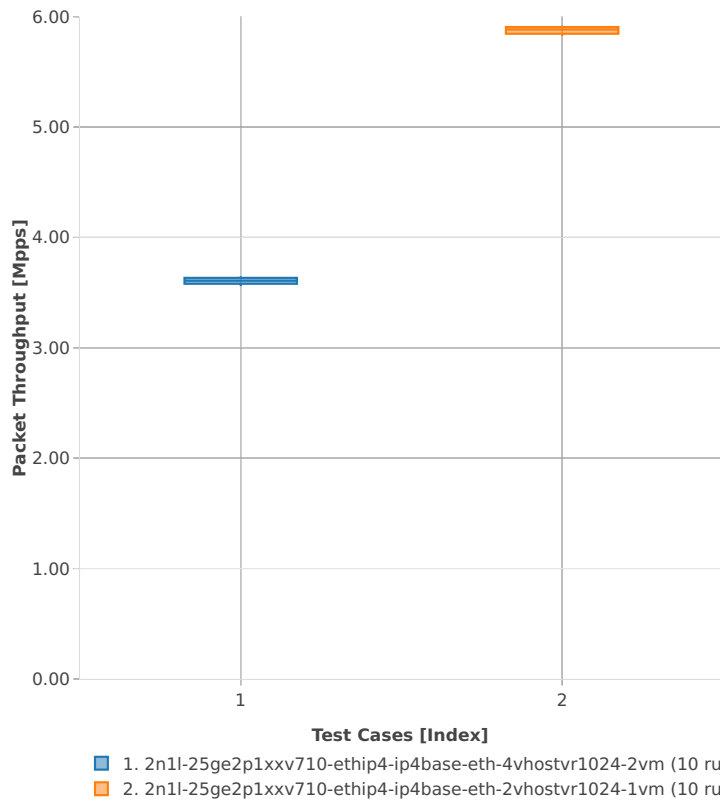
Packet Throughput: vhost-ip4-2n-skx-xxv710-64b-2t1c-base_and_scale-pdr
