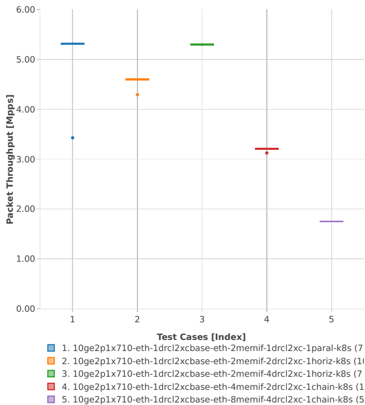
Packet Throughput: k8s-memif-3n-hsw-x710-64b-1t1c-base_and_scale-l2xc-p
