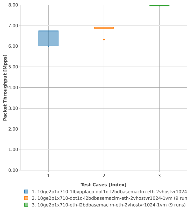
Packet Throughput: vhost-l2sw-3n-hsw-x710-64b-2t2c-base_and_scale-pdr
