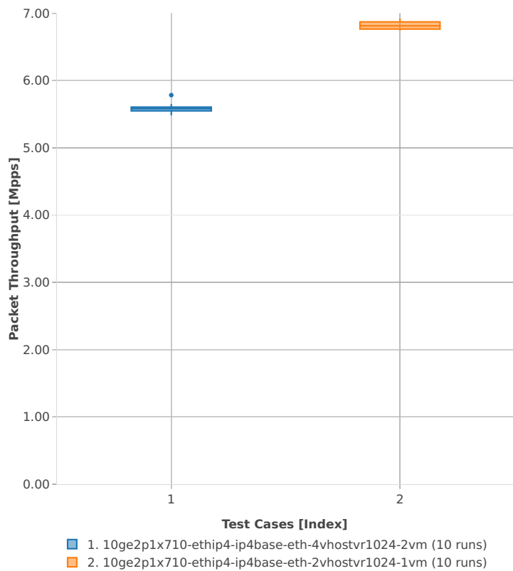
Packet Throughput: vhost-ip4-3n-skx-x710-64b-4t2c-base_and_scale-pdr
