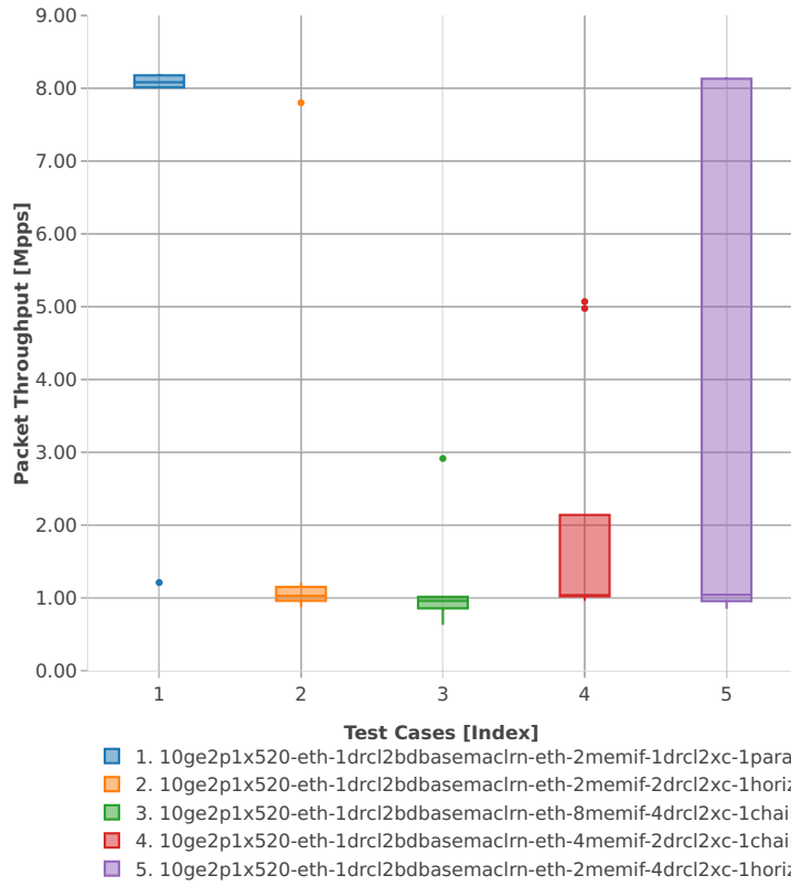
Packet Throughput: k8s-memif-3n-hsw-x520-64b-2t2c-base_and_scale-l2bd-ndr
