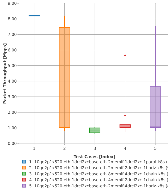
Packet Throughput: k8s-memif-3n-hsw-x520-64b-2t2c-base_and_scale-l2xc-n
