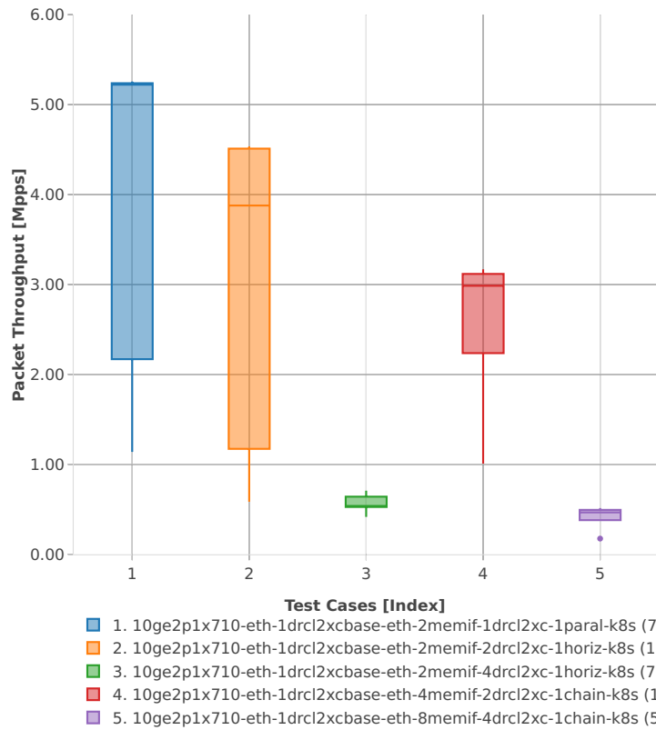
Packet Throughput: k8s-memif-3n-hsw-x710-64b-1t1c-base_and_scale-l2xc-n
