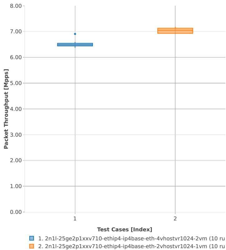
Packet Throughput: vhost-ip4-2n-skx-xxv710-64b-4t2c-base_and_scale-pdr
