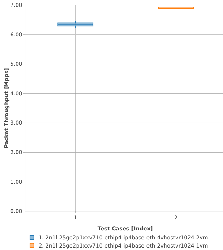
Packet Throughput: vhost-ip4-2n-skx-xxv710-64b-4t2c-base_and_scale-ndr
