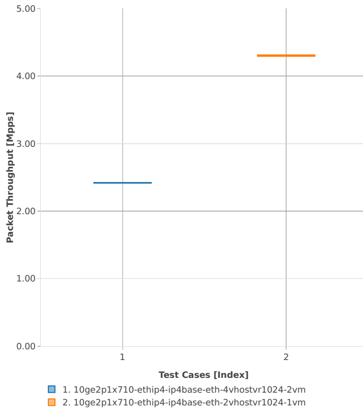
Packet Throughput: vhost-ip4-3n-hsw-x710-64b-1t1c-base_and_scale-pdr
