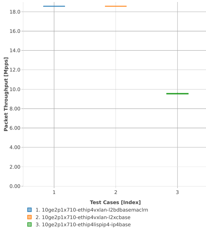
Packet Throughput: ip4tun-3n-skx-x710-64b-4t2c-base_and_features-ndr
