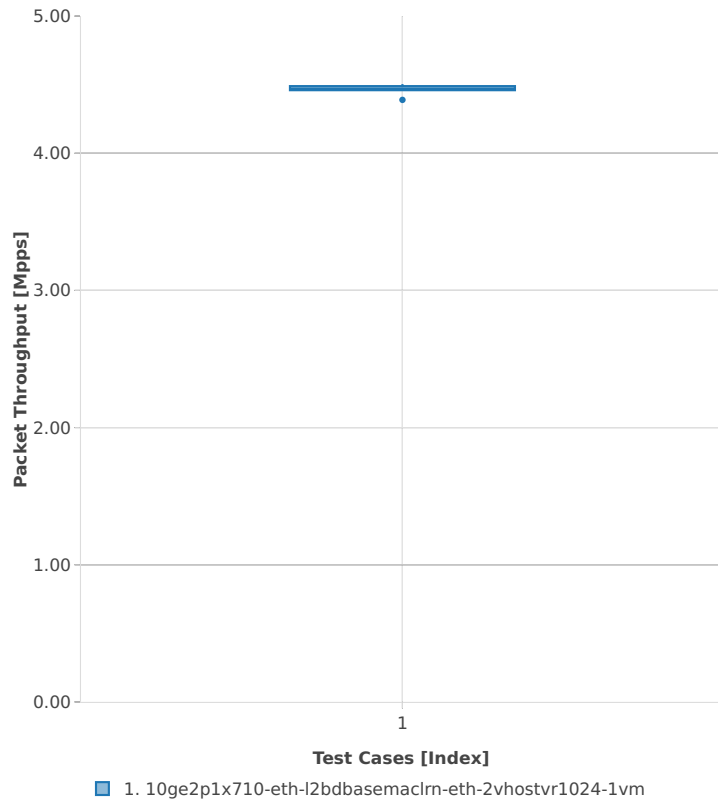
Packet Throughput: vhost-l2sw-3n-hsw-x710-64b-1t1c-base_and_scale-ndr
