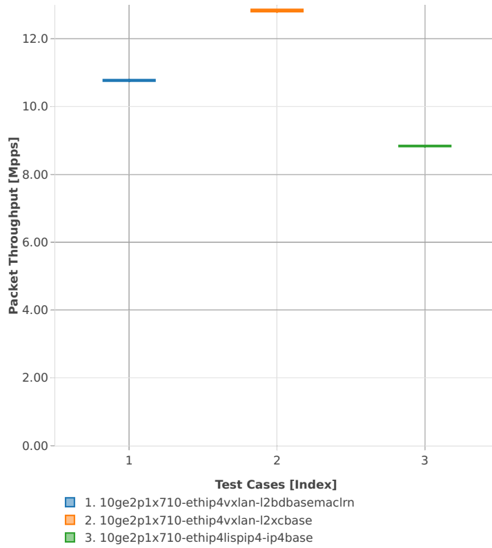
Packet Throughput: ip4tun-3n-skx-x710-64b-2t1c-base_and_features-ndr
