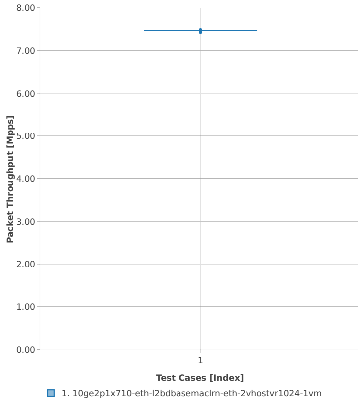
Packet Throughput: vhost-l2sw-3n-hsw-x710-64b-2t2c-base_and_scale-ndr
