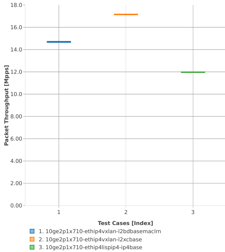
Packet Throughput: ip4tun-3n-hsw-x710-64b-2t2c-base_and_features-ndr
