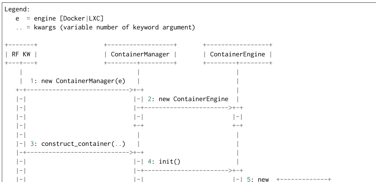
Sequential diagram that illustrates the creation of a single container.
